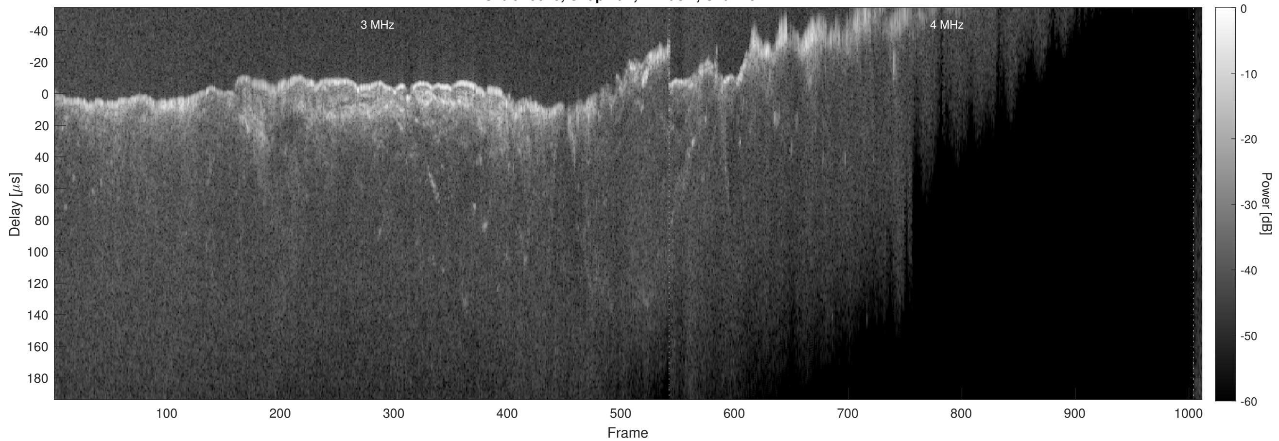
Orbit 10646, Chapman, Window, Channel 2
