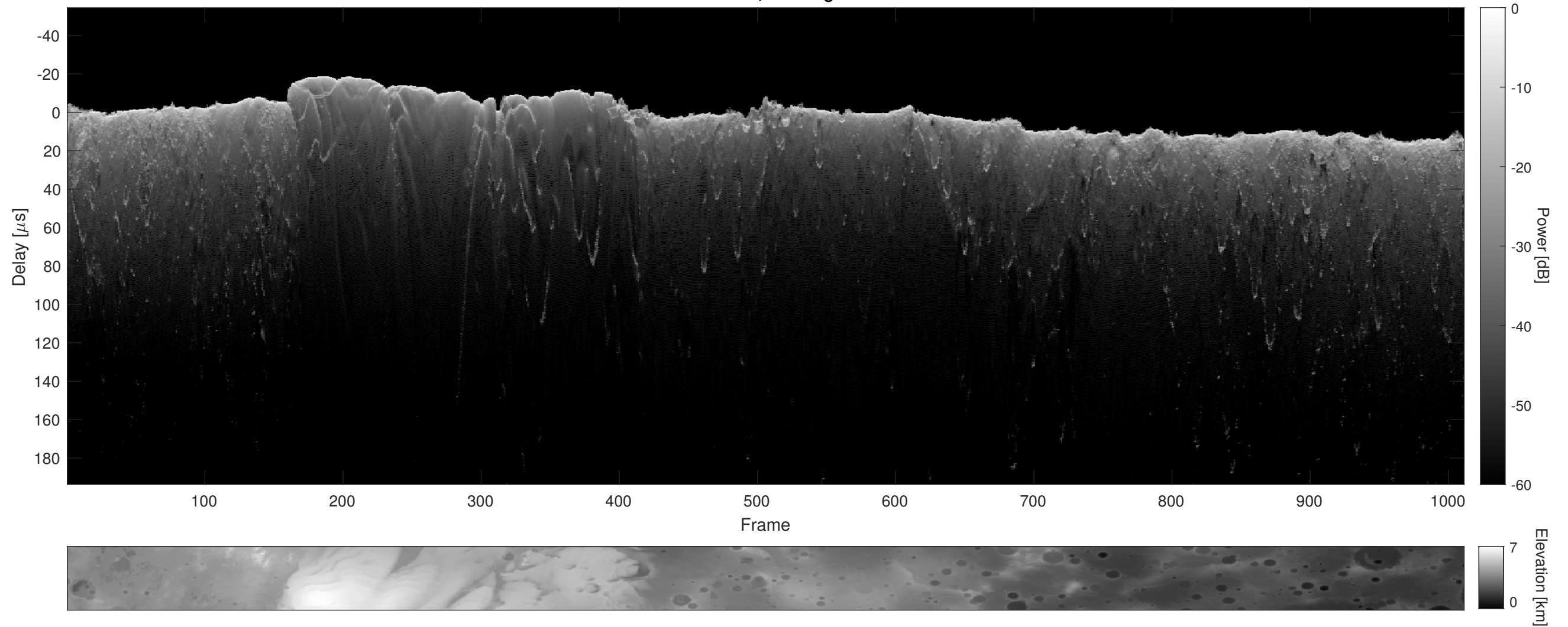
Orbit 10646, Cluttergram
