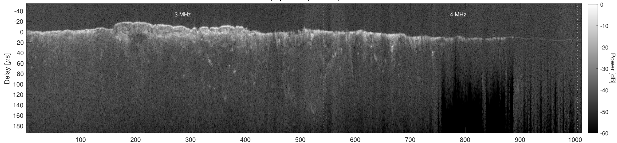
Orbit 10646, Cluttergram
