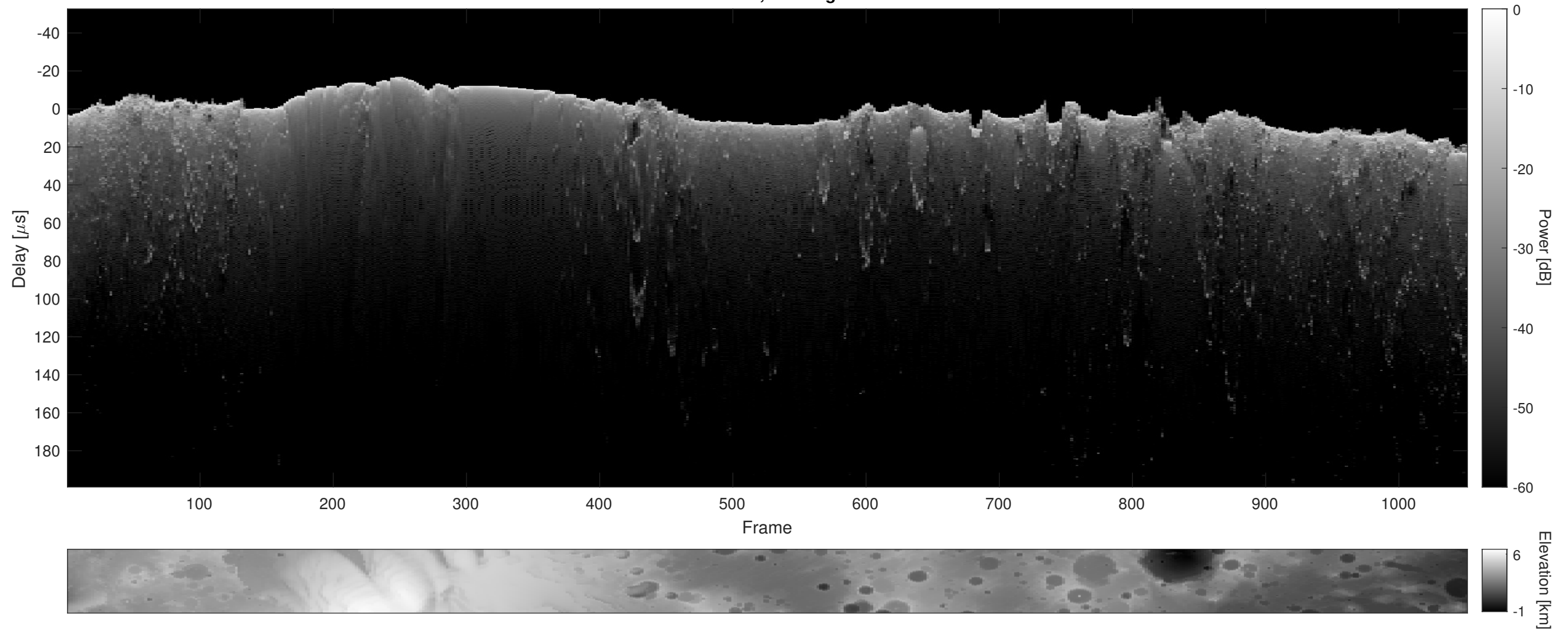
Orbit 10649, Cluttergram
