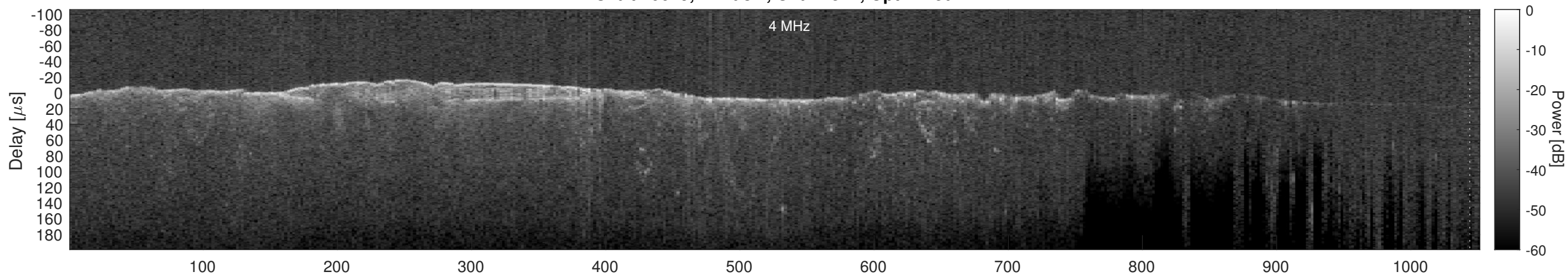
Orbit 10649, Cluttergram
