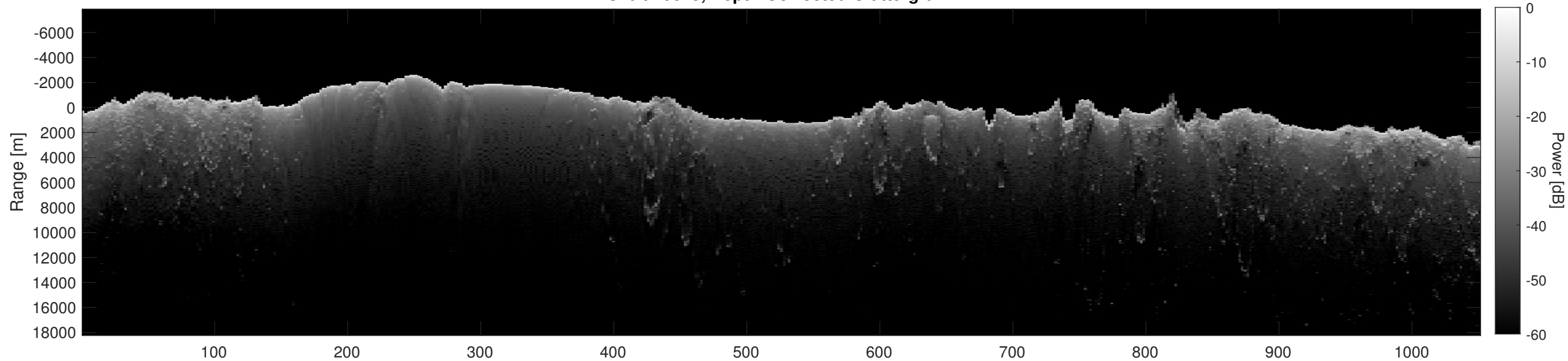
Orbit 10649, Depth-Corrected Cluttergram
