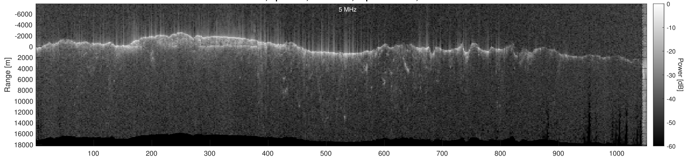
Orbit 10649, Optimized, No Window, Depth-Corrected, Channel 2
