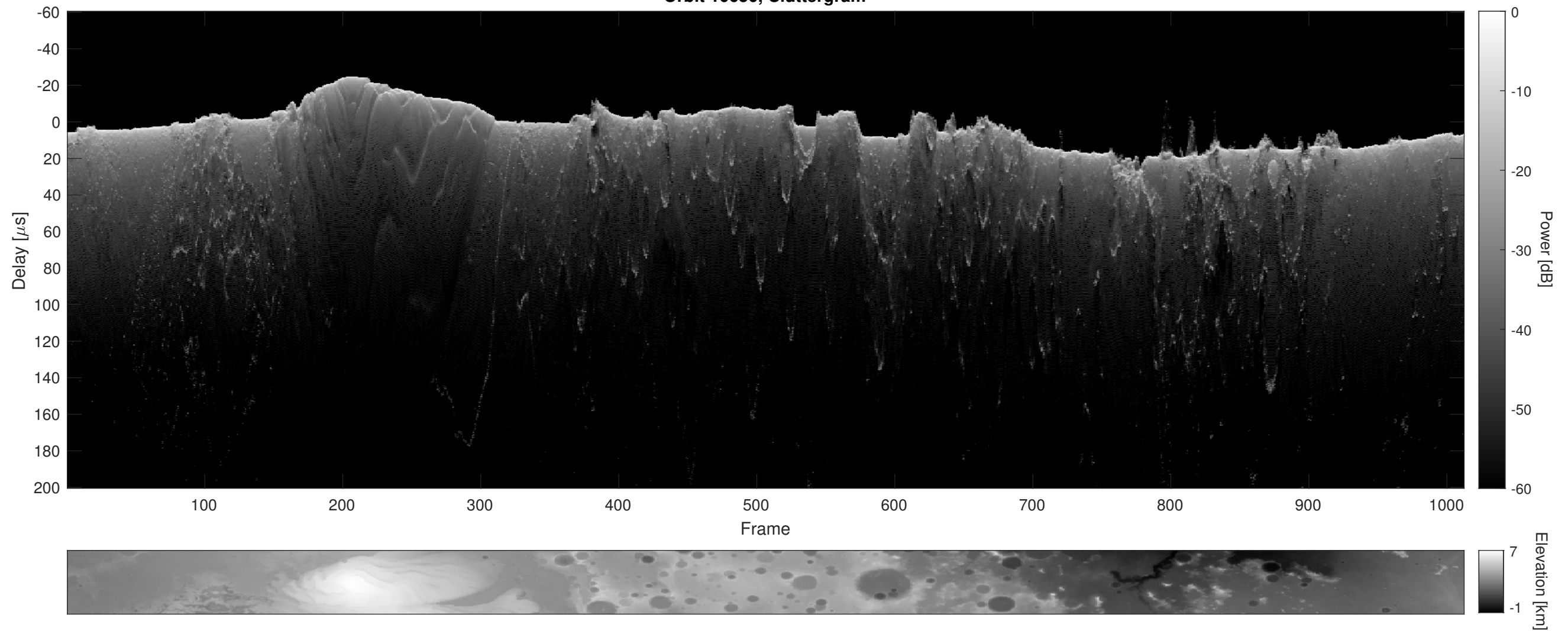
Orbit 10650, Cluttergram
