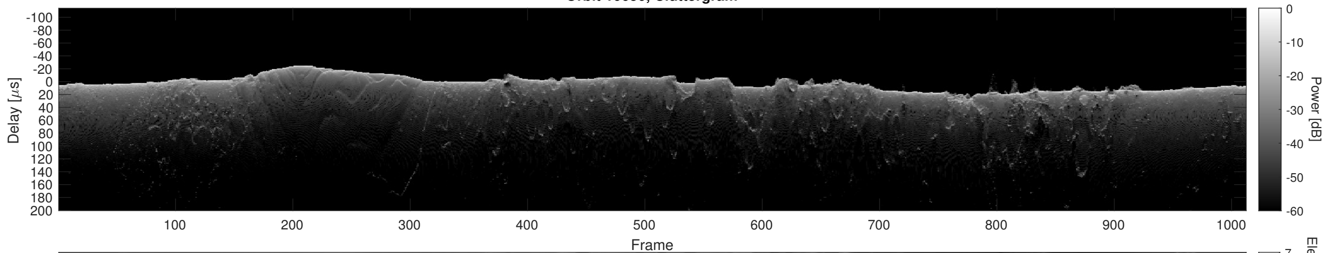
Orbit 10650, Cluttergram
