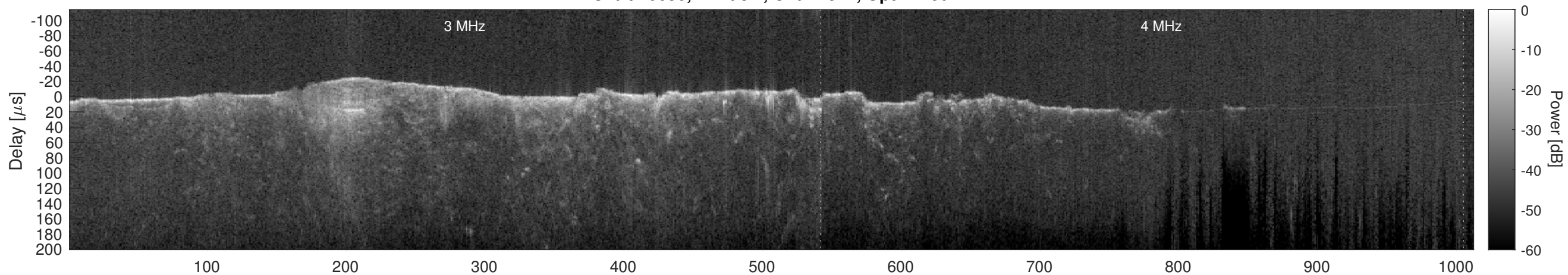
Orbit 10650, Cluttergram
