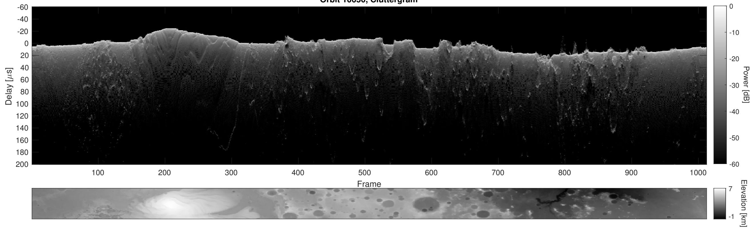
Orbit 10650, Cluttergram
