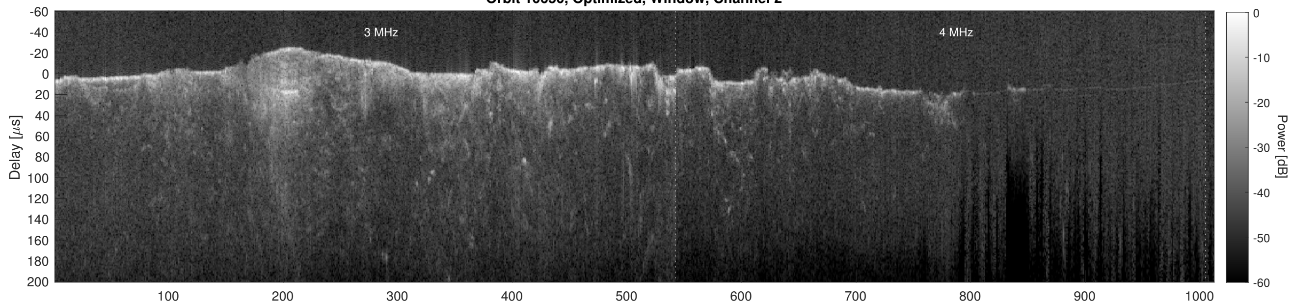
Orbit 10650, Cluttergram
