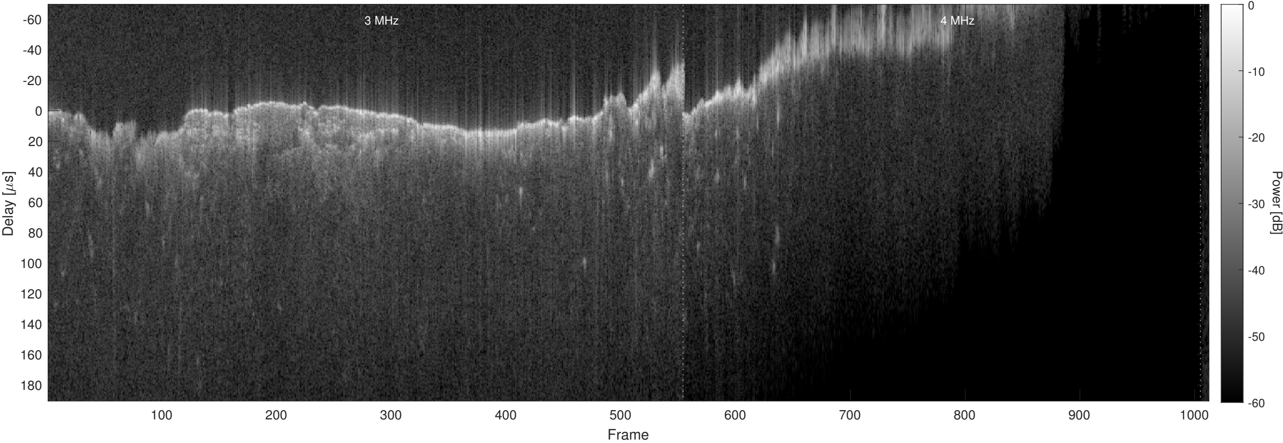
Orbit 10652, Chapman, No Window, Channel 2
