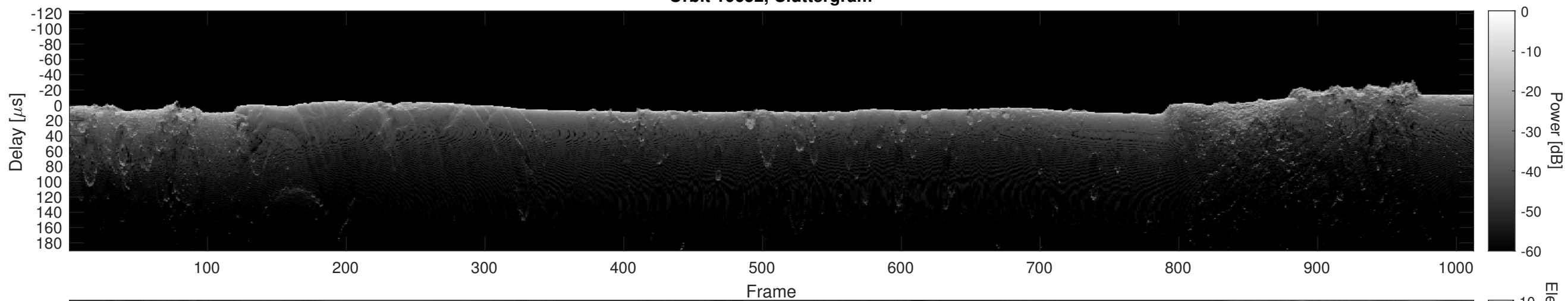
Orbit 10652, Cluttergram
