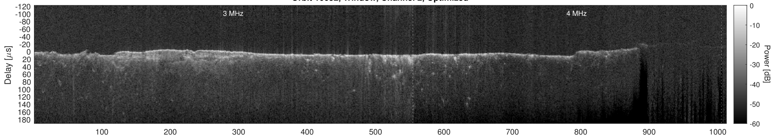
Orbit 10652, Cluttergram
