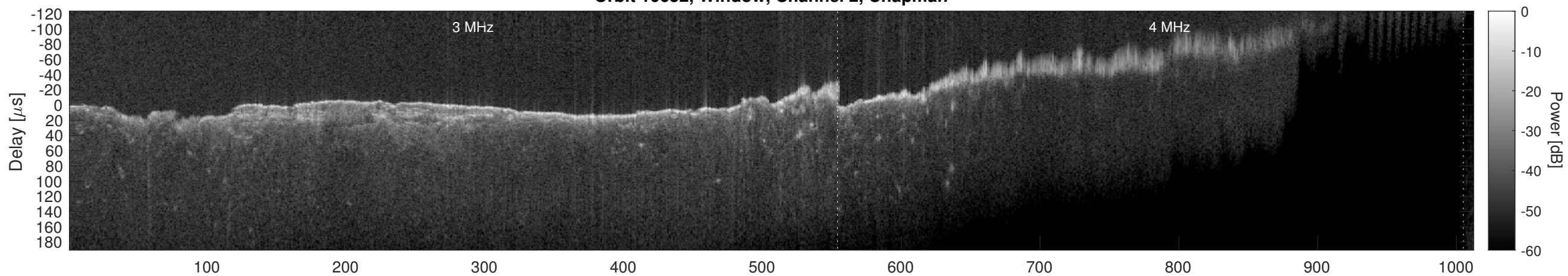
Orbit 10652, Window, Channel 2, Optimized
