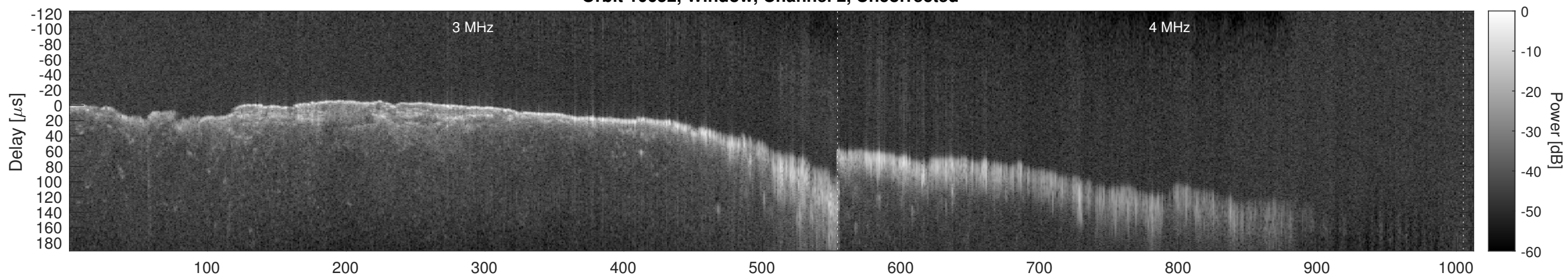
Orbit 10652, Window, Channel 2, Chapman
