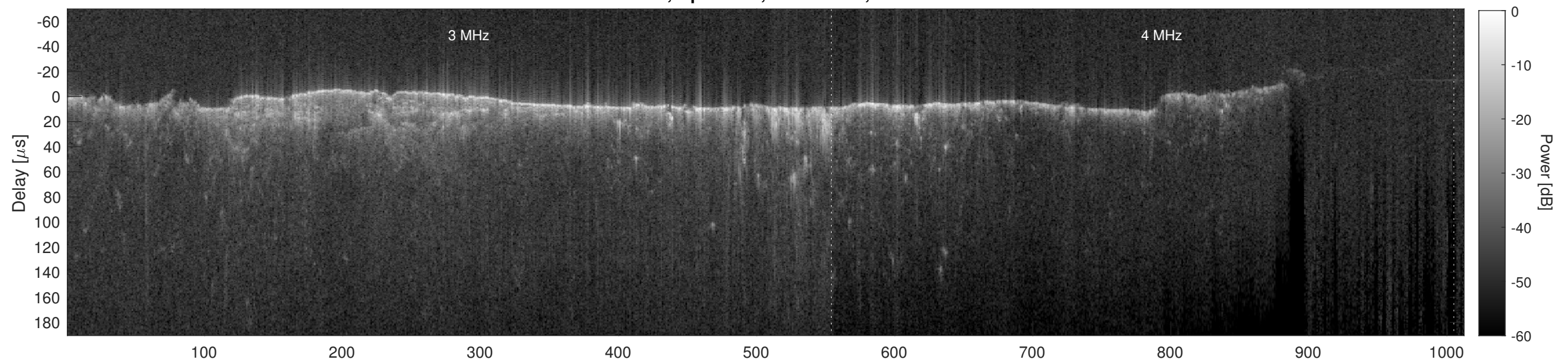
Orbit 10652, Cluttergram
