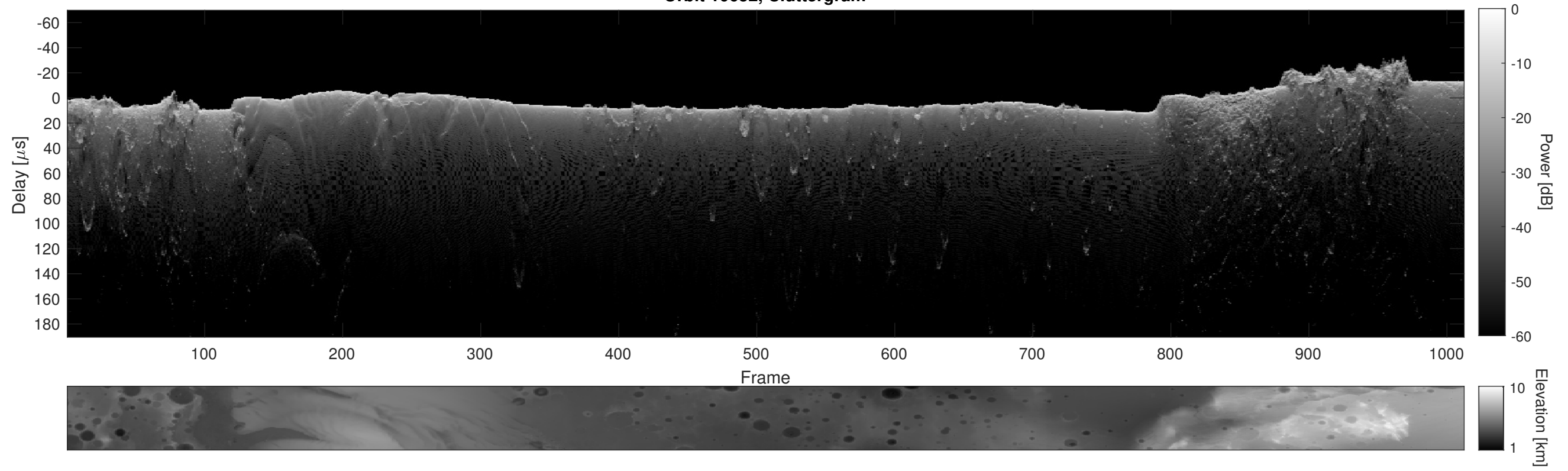
Orbit 10652, Cluttergram
