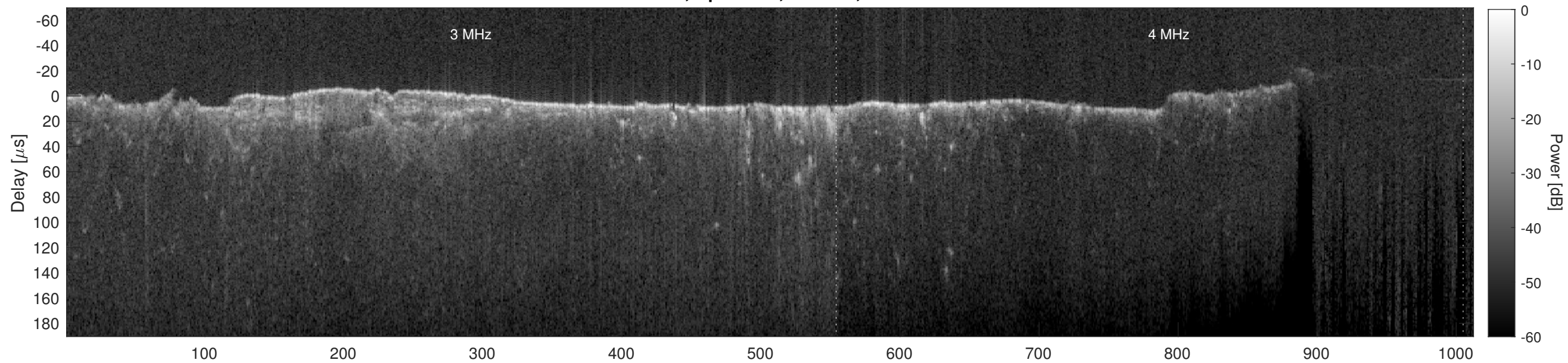
Orbit 10652, Cluttergram
