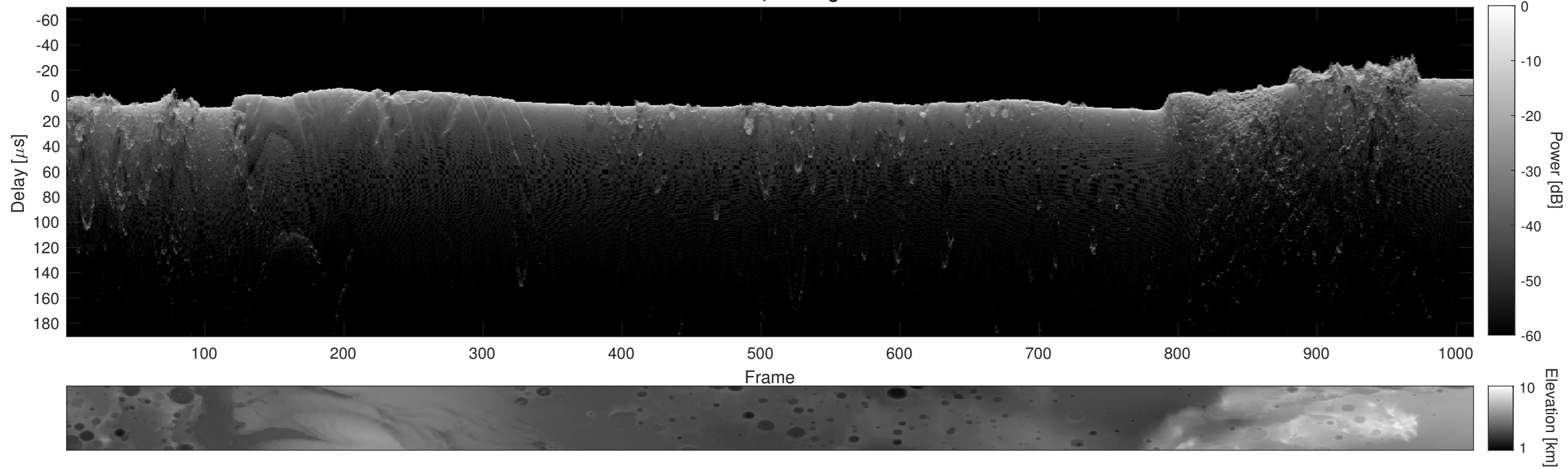
Orbit 10652, Cluttergram
