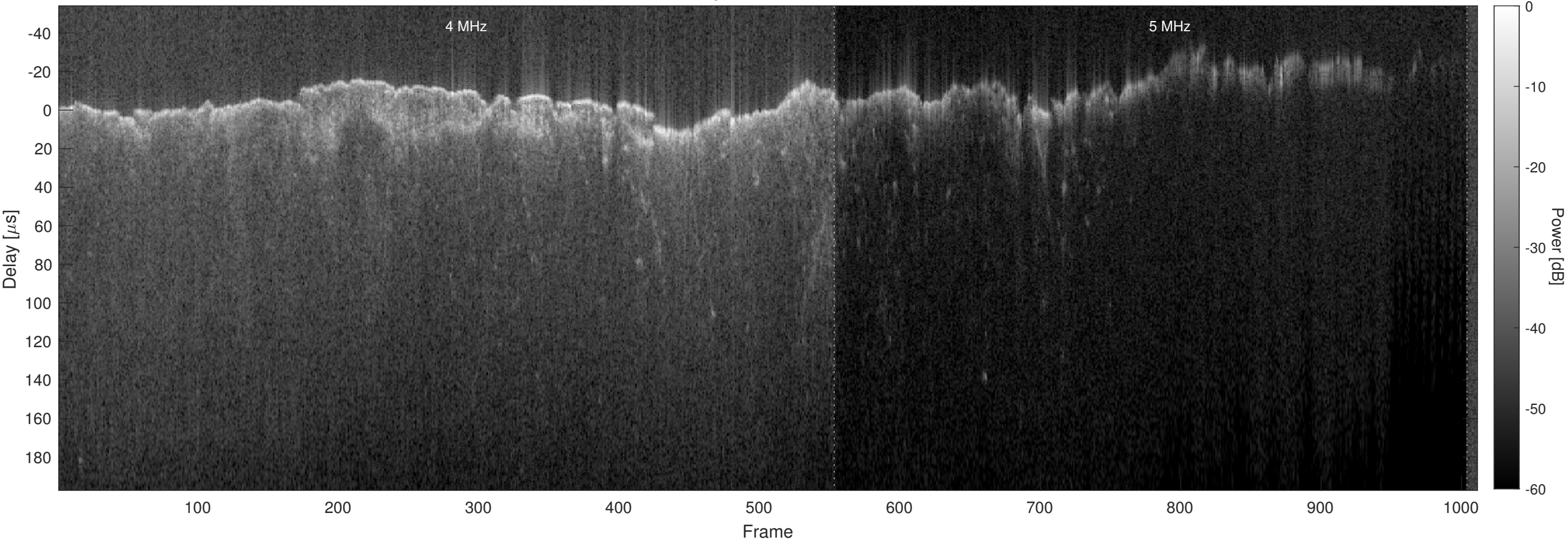
Orbit 10653, Chapman, No Window, Channel 2
