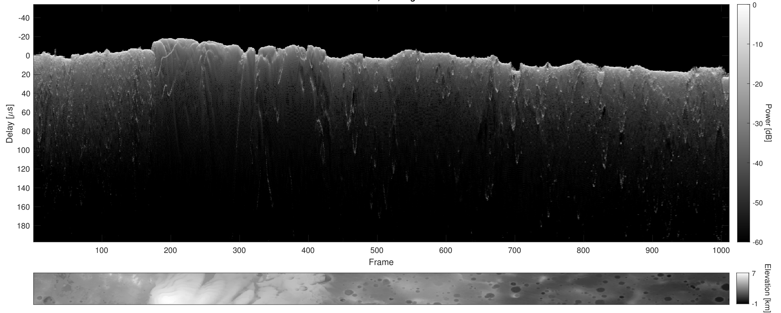
Orbit 10653, Cluttergram
