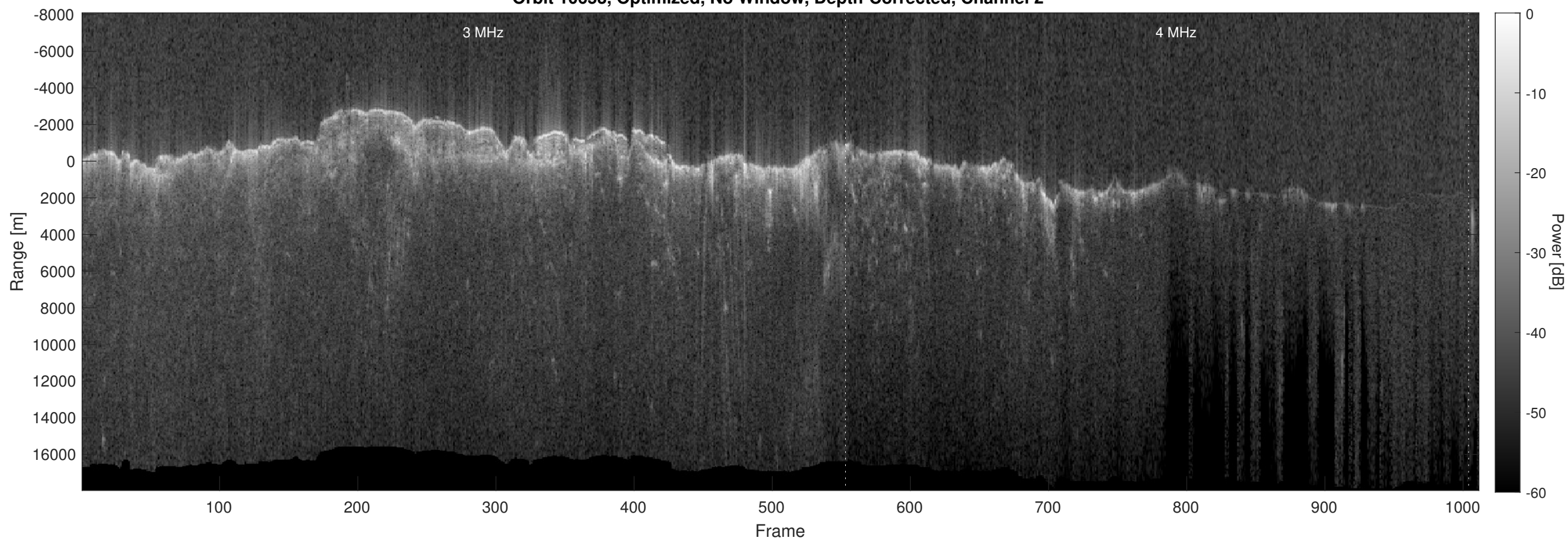
Orbit 10653, Optimized, No Window, Depth-Corrected, Channel 2
