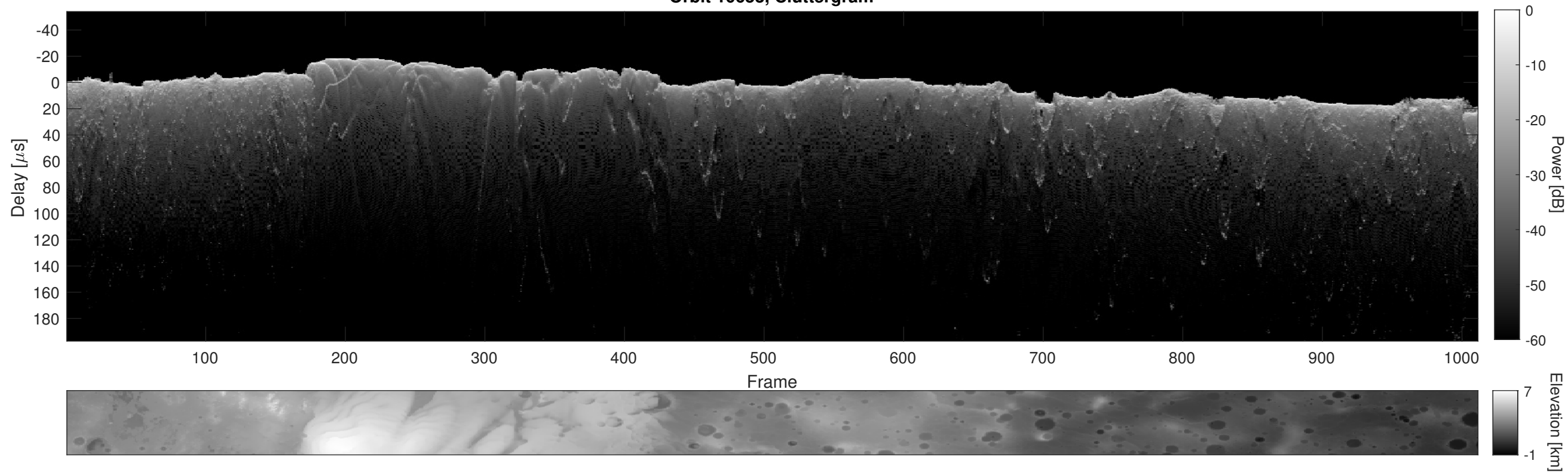
Orbit 10653, Cluttergram
