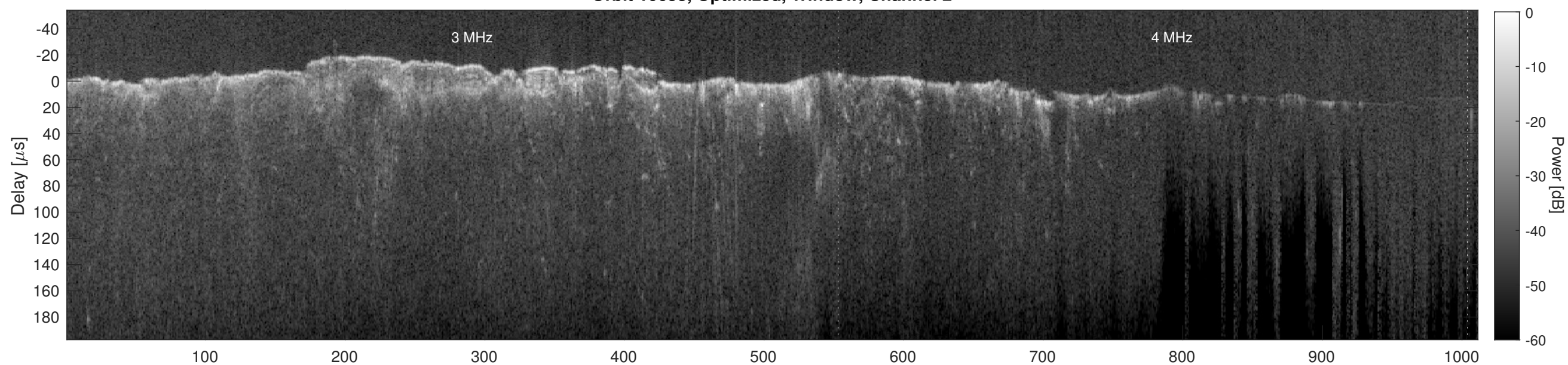
Orbit 10653, Cluttergram
