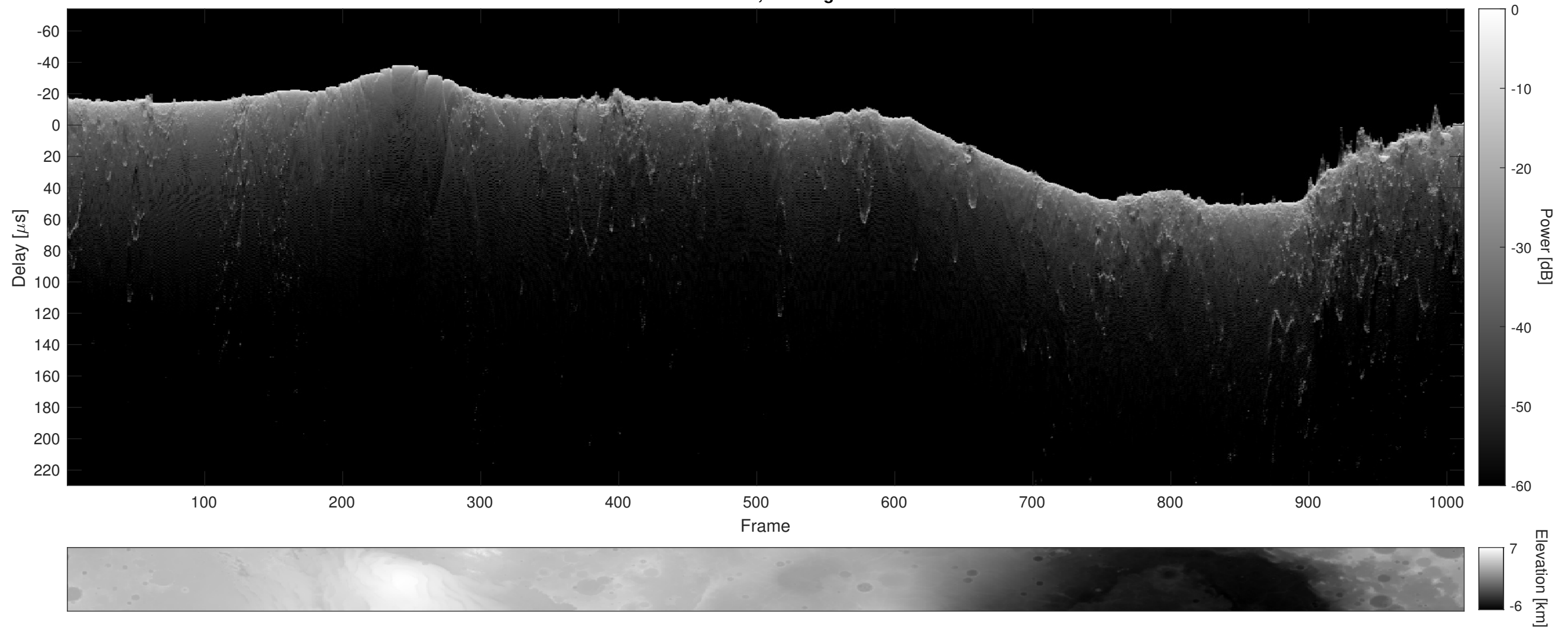
Orbit 10654, Cluttergram
