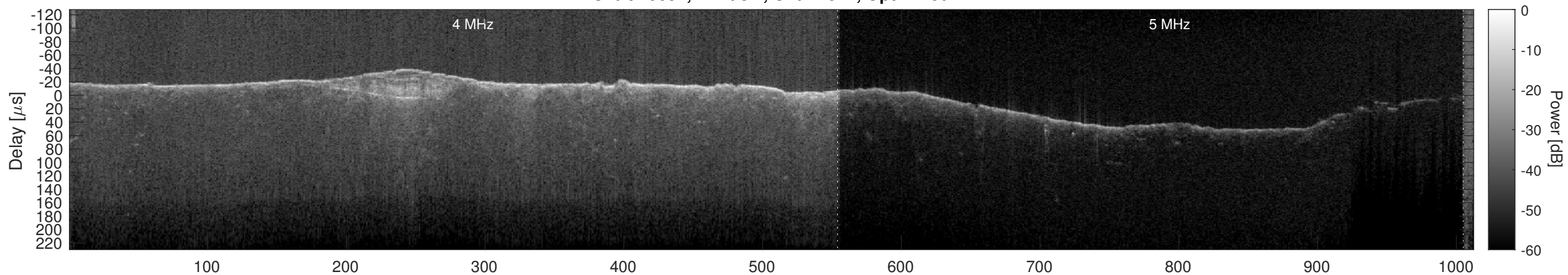
Orbit 10654, Cluttergram
