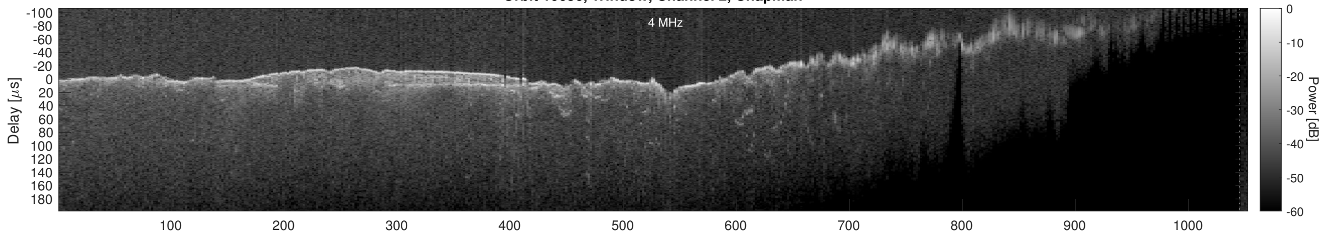
Orbit 10656, Window, Channel 2, Optimized
