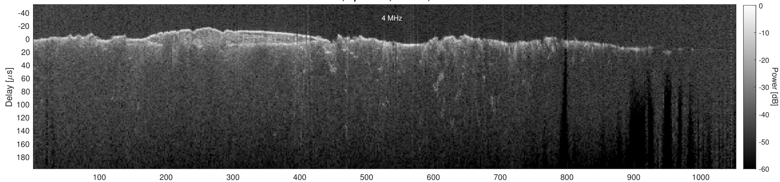
Orbit 10656, Cluttergram
