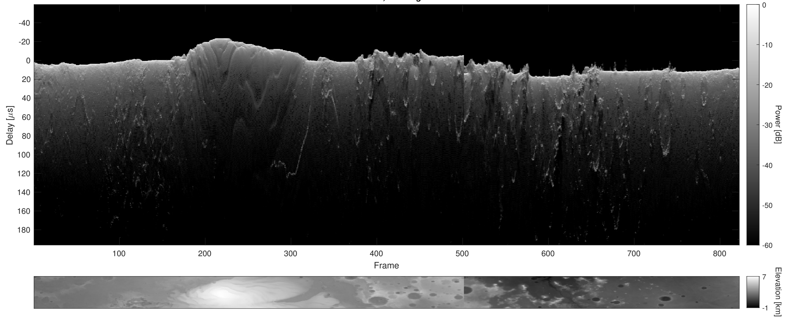
Orbit 10657, Cluttergram
