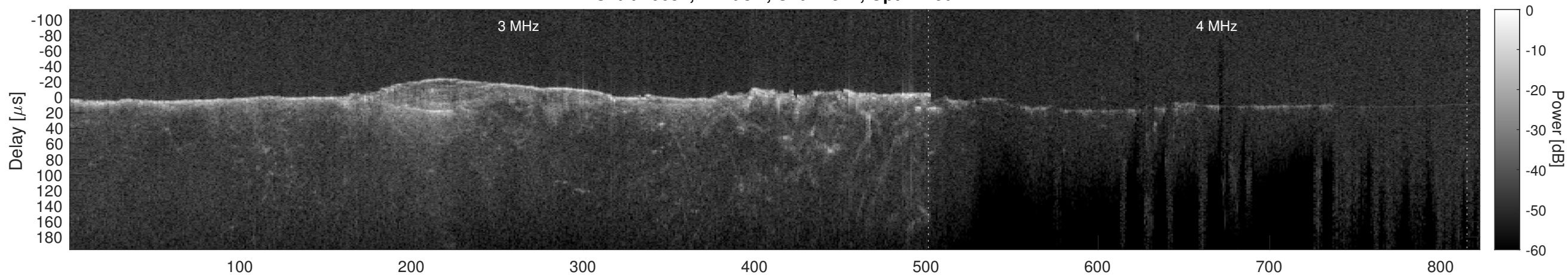
Orbit 10657, Cluttergram
