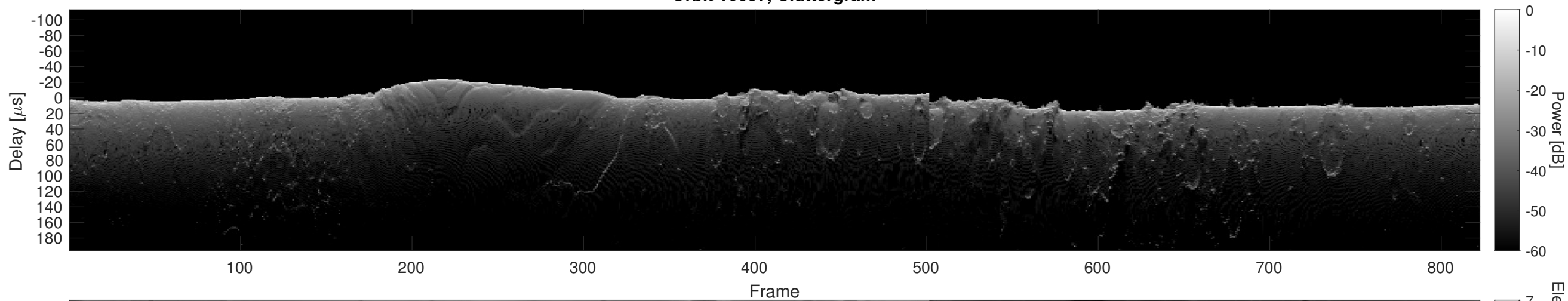
Orbit 10657, Cluttergram
