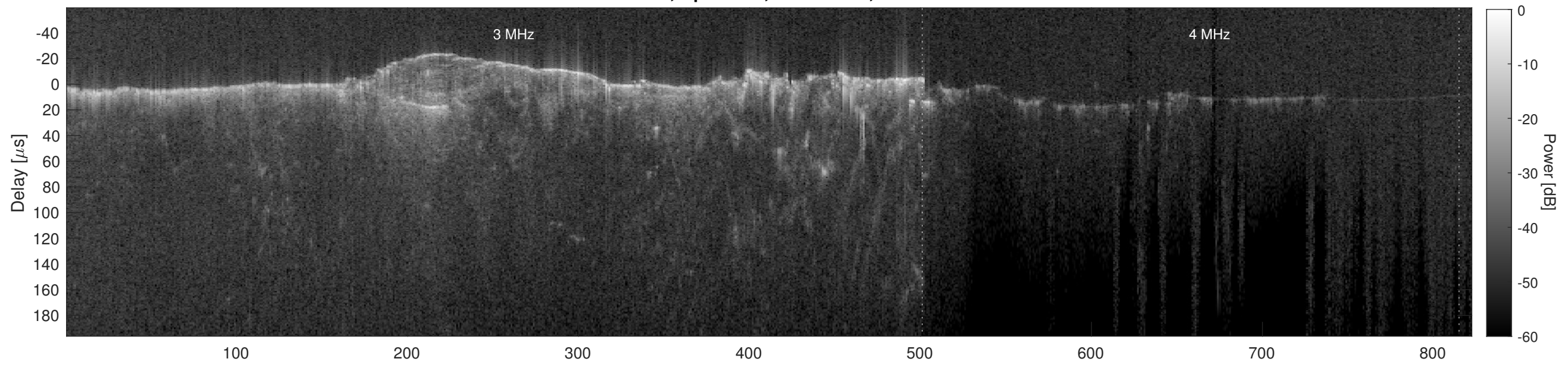
Orbit 10657, Cluttergram
