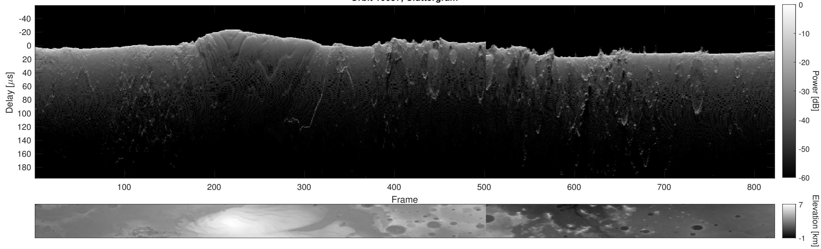
Orbit 10657, Cluttergram
