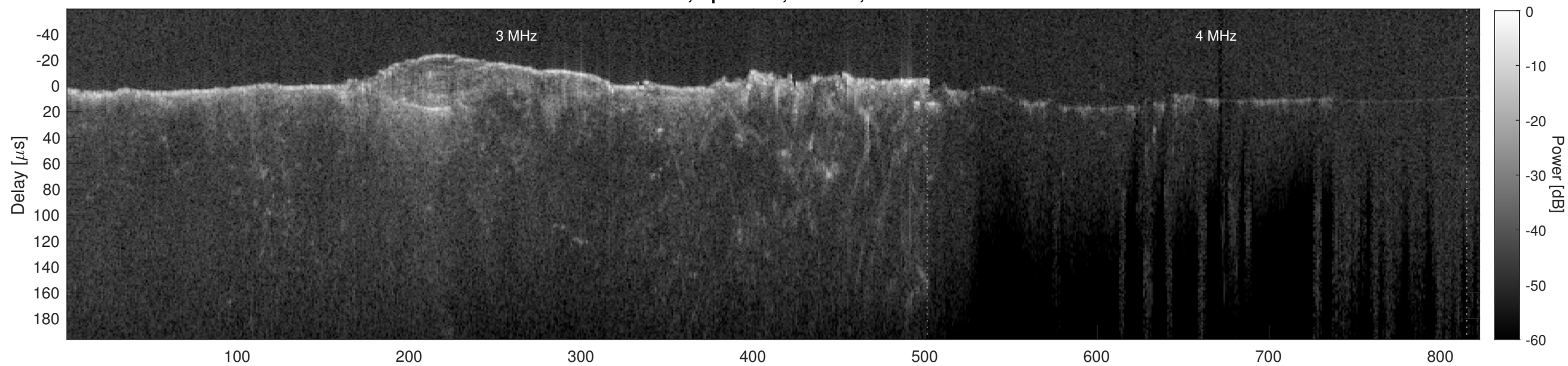
Orbit 10657, Cluttergram
