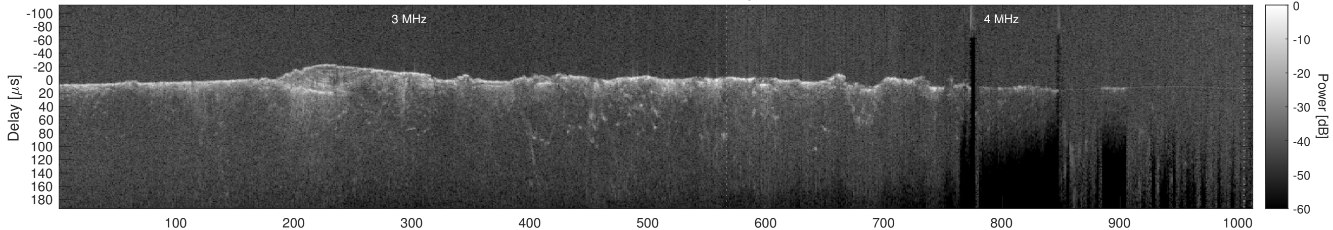
Orbit 10664, Cluttergram
