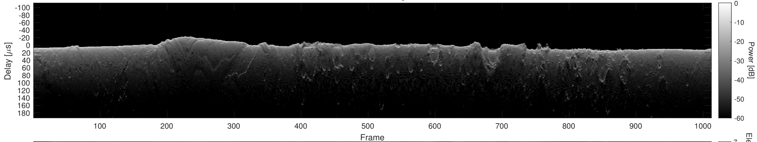
Orbit 10664, Cluttergram
