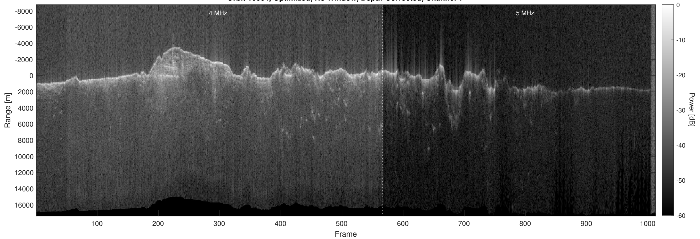
Orbit 10664, Optimized, No Window, Depth-Corrected, Channel 2
