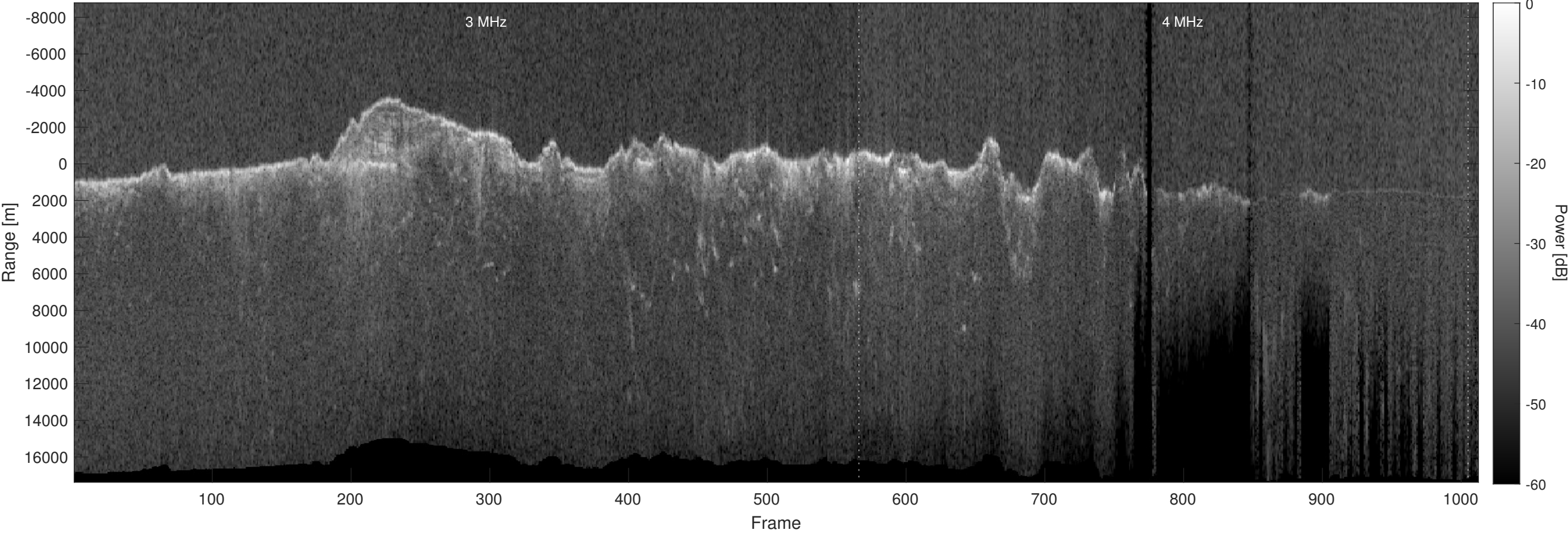
Orbit 10664, Optimized, Window, Depth-Corrected, Channel 2
