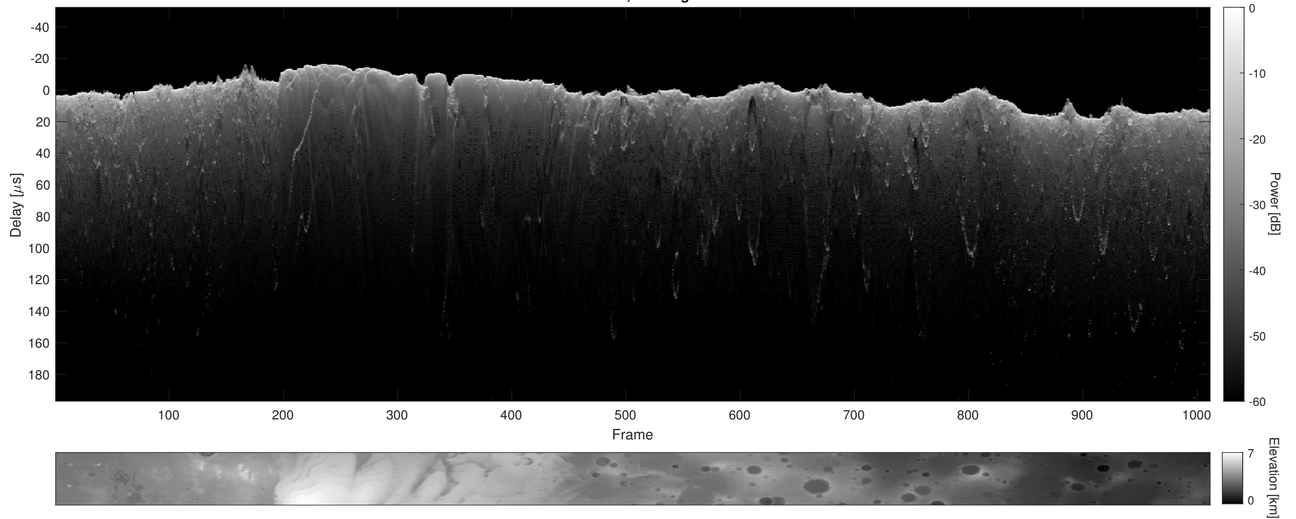
Orbit 10667, Cluttergram
