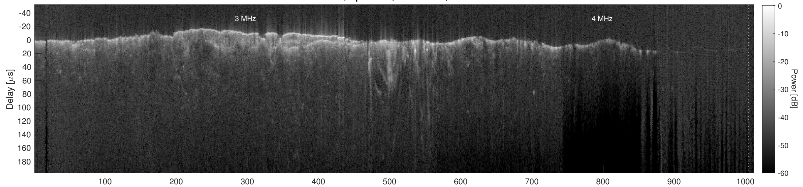
Orbit 10667, Cluttergram
