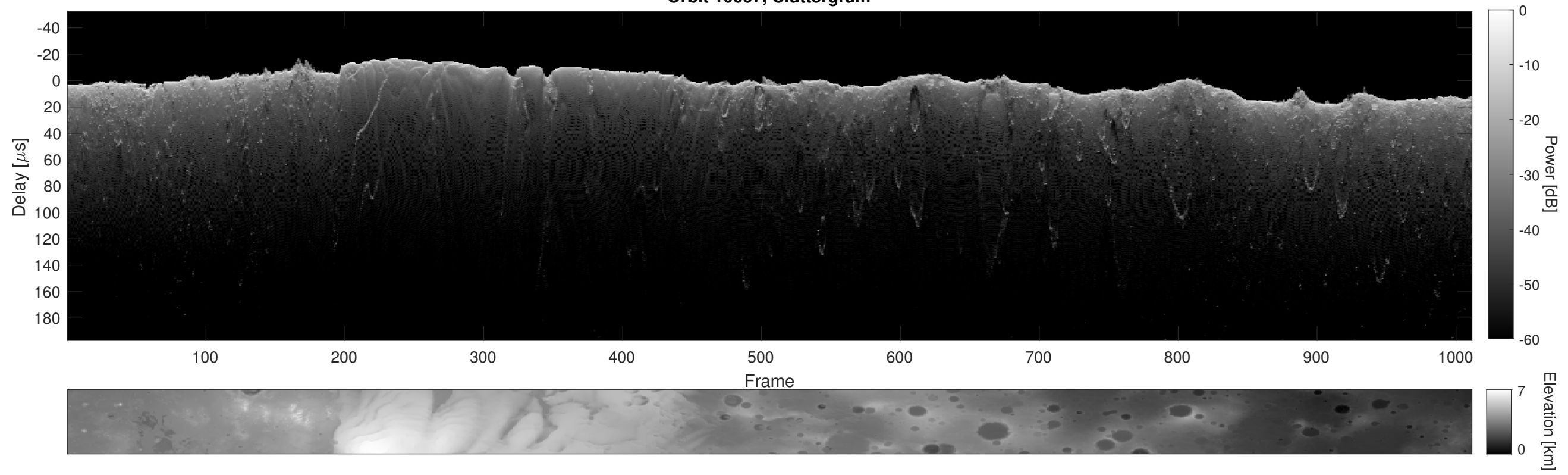
Orbit 10667, Cluttergram
