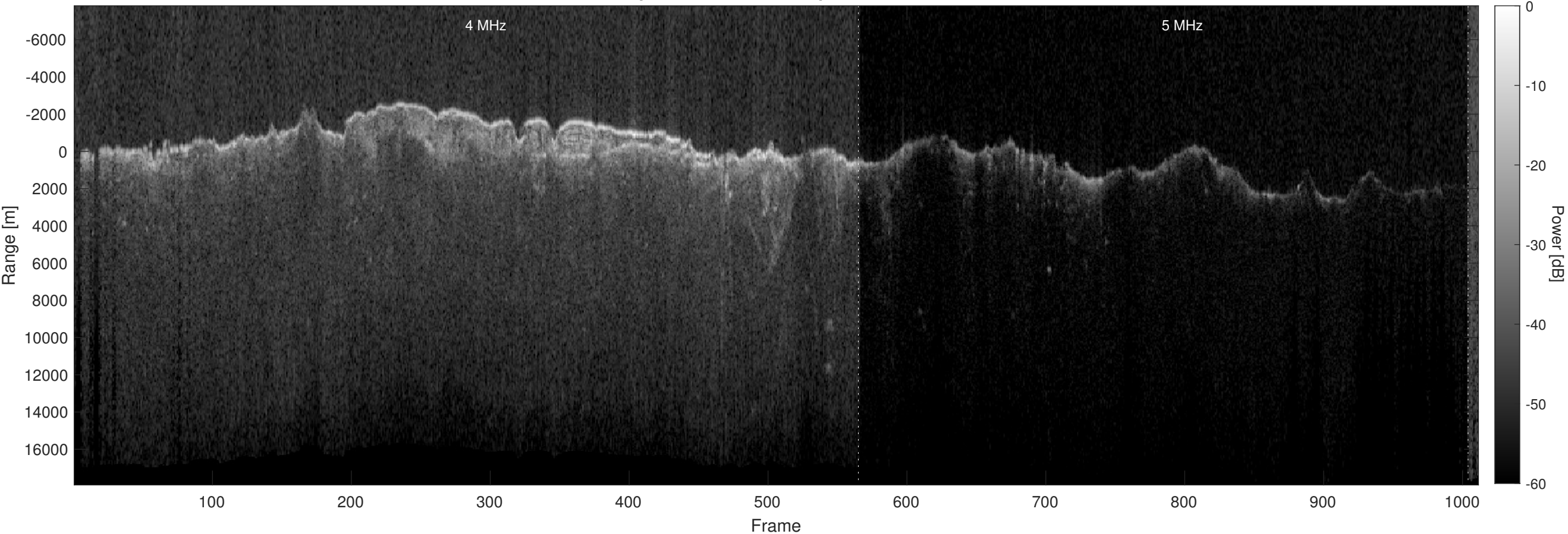
Orbit 10667, Optimized, Window, Depth-Corrected, Channel 2
