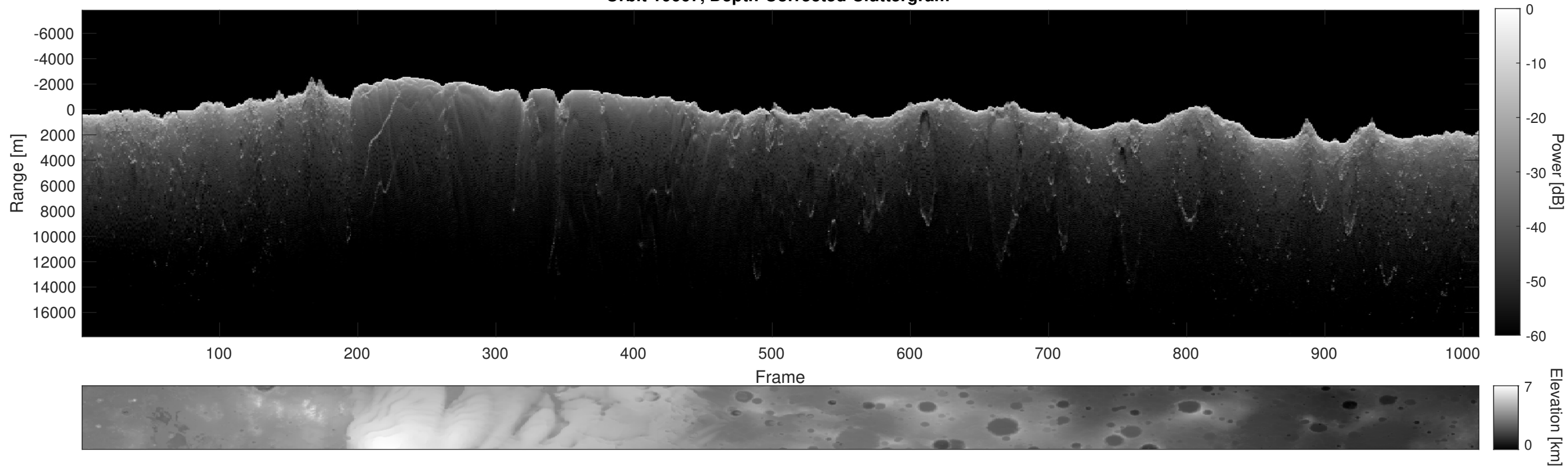
Orbit 10667, Depth-Corrected Cluttergram
