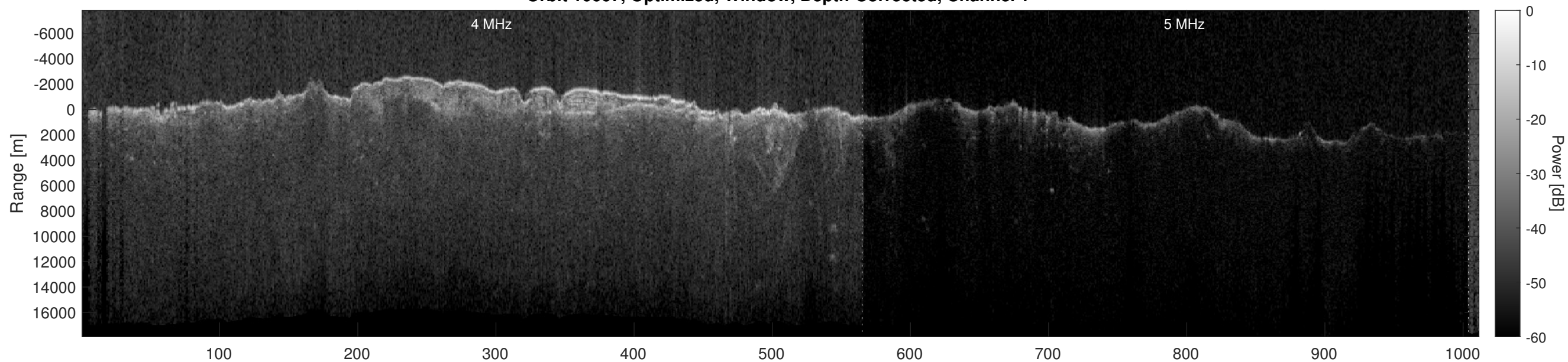
Orbit 10667, Optimized, Window, Depth-Corrected, Channel 2
