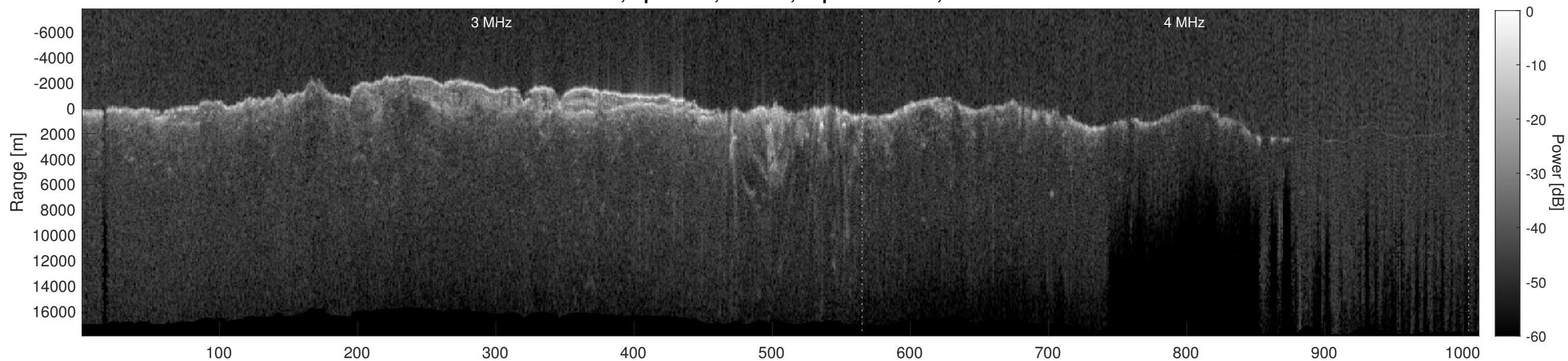
Orbit 10667, Depth-Corrected Cluttergram
