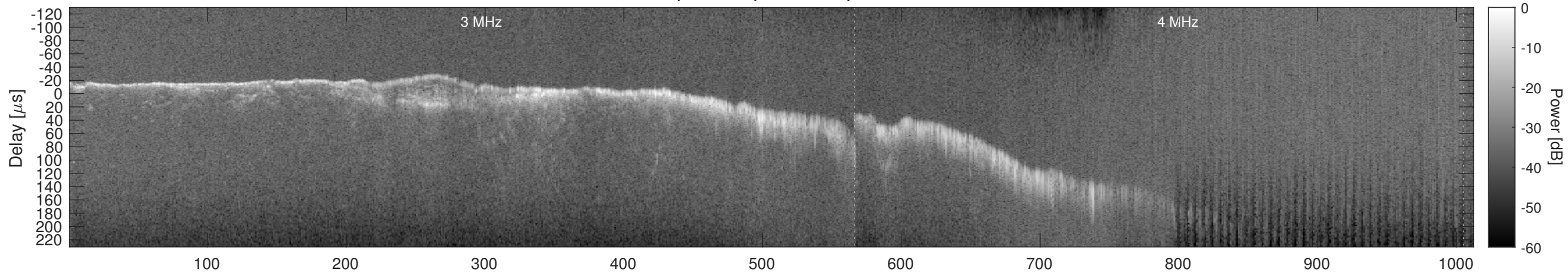
Orbit 10668, Window, Channel 2, Chapman
