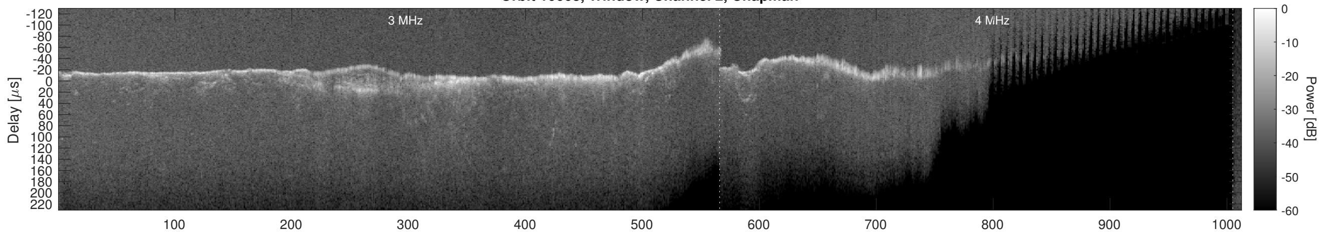
Orbit 10668, Window, Channel 2, Optimized
