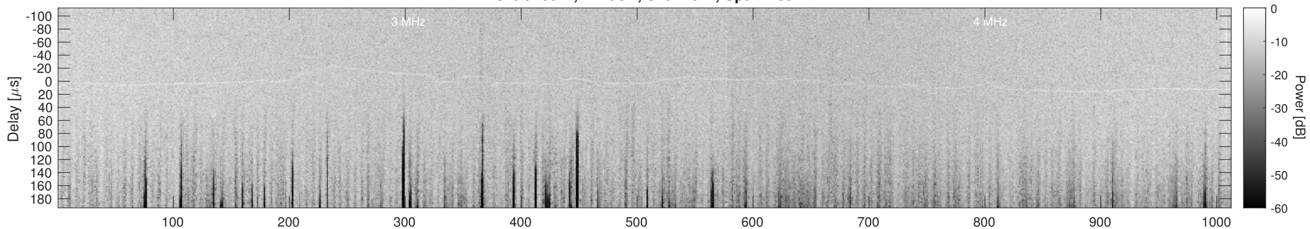
Orbit 10671, Cluttergram
