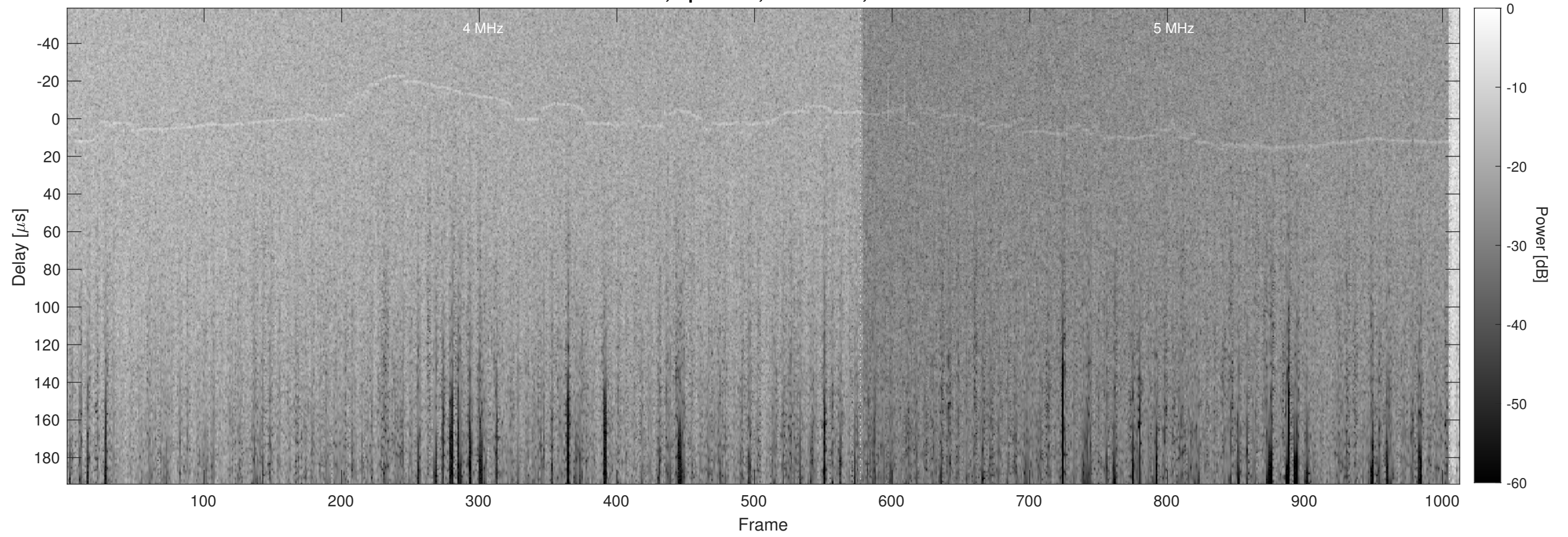
Orbit 10671, Optimized, No Window, Channel 2
