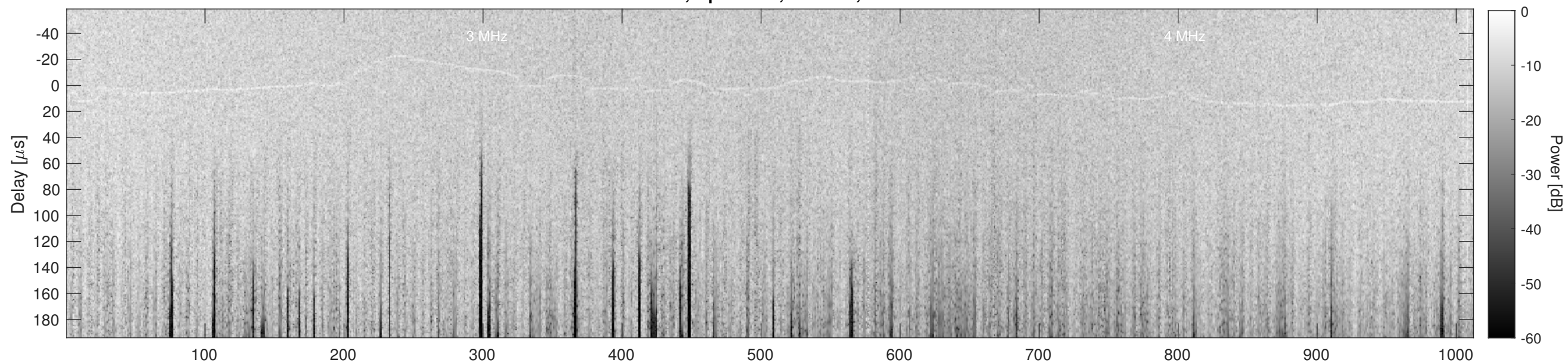
Orbit 10671, Cluttergram
