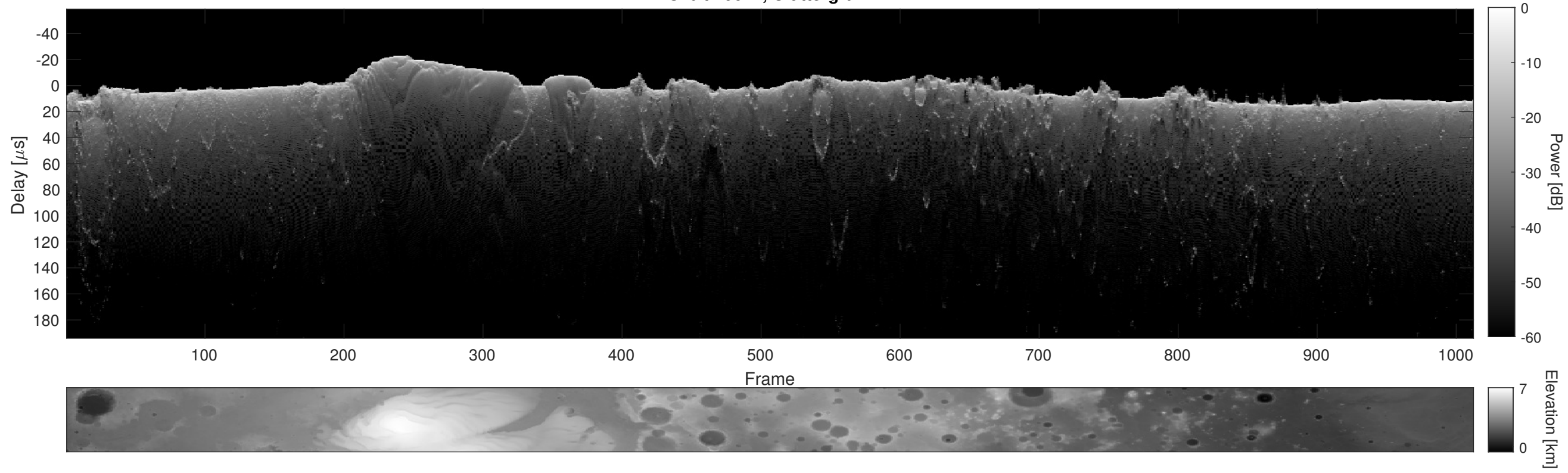
Orbit 10671, Cluttergram
