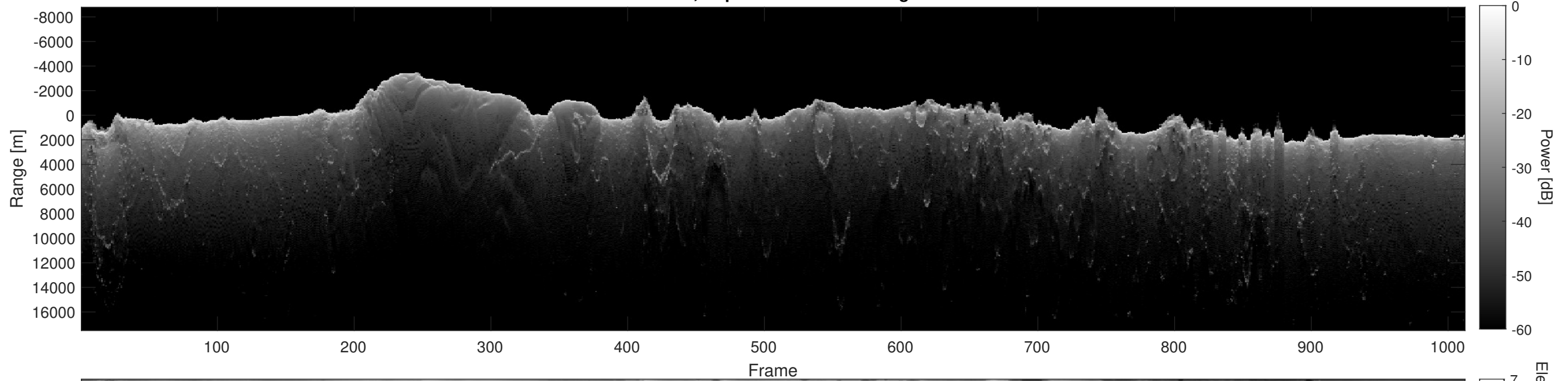
Orbit 10671, Depth-Corrected Cluttergram
