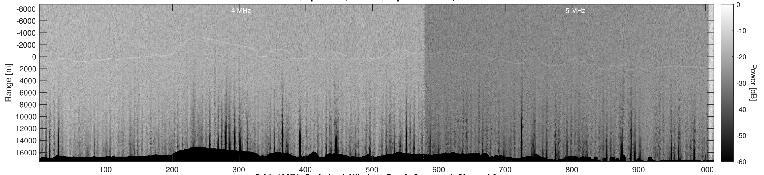
Orbit 10671, Optimized, Window, Depth-Corrected, Channel 2
