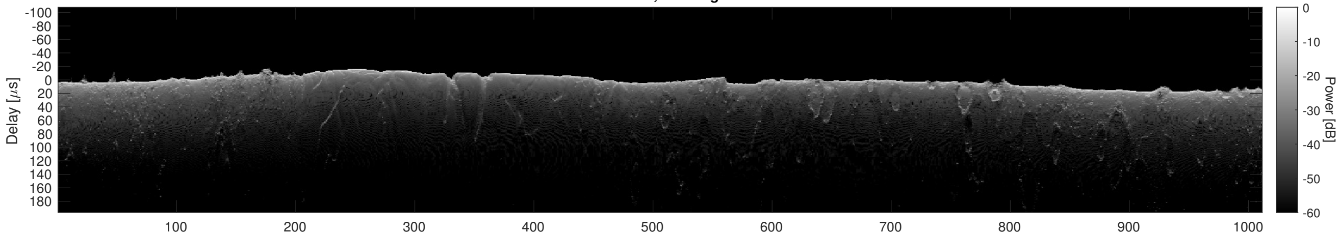
Orbit 10674, Cluttergram
