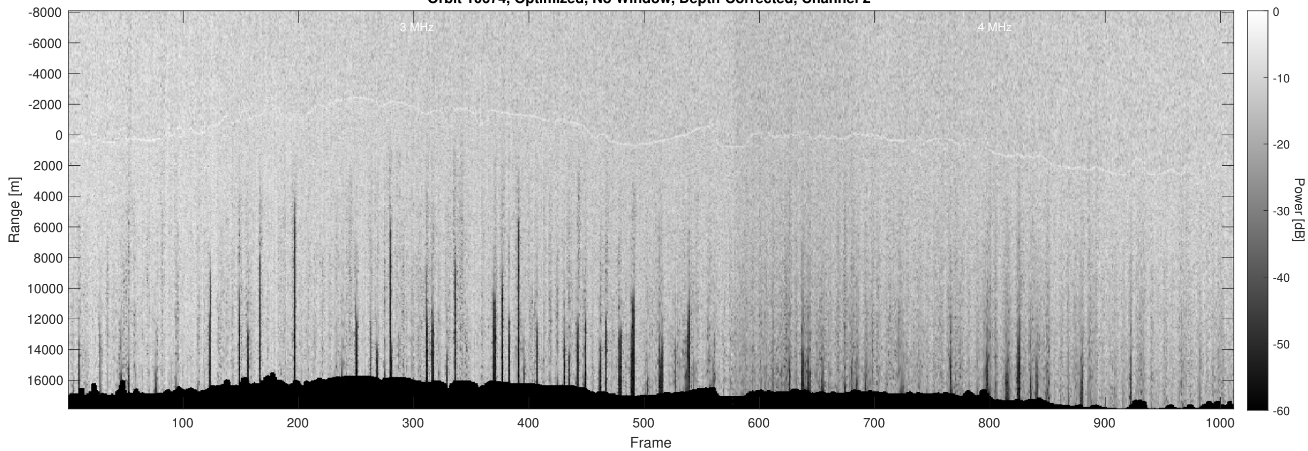
Orbit 10674, Optimized, No Window, Depth-Corrected, Channel 2
