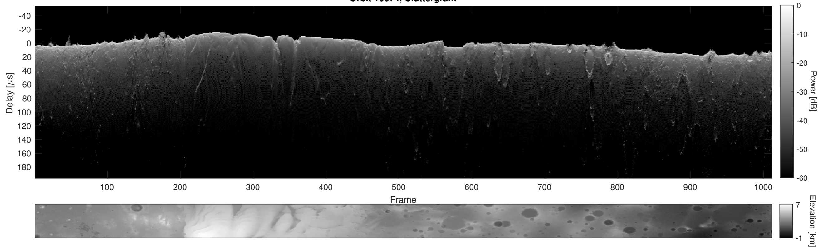
Orbit 10674, Cluttergram
