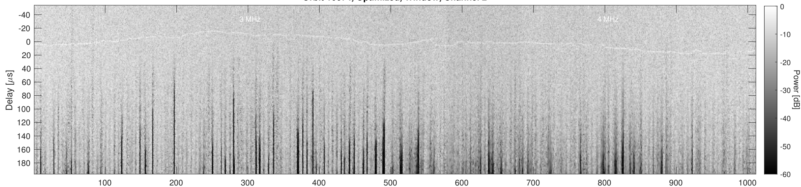
Orbit 10674, Cluttergram
