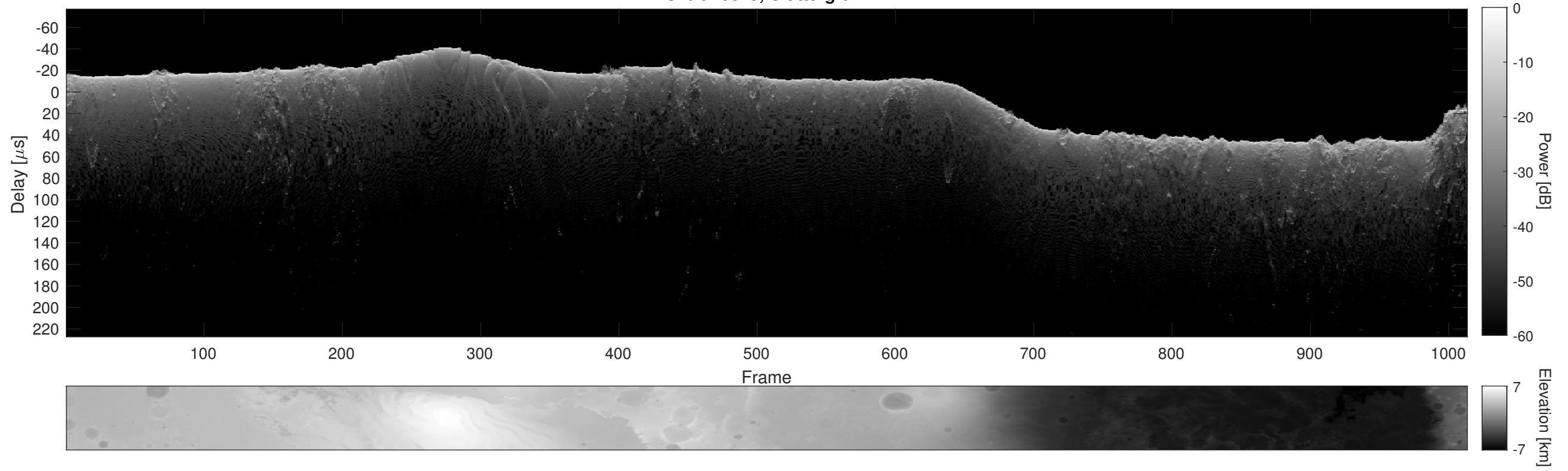
Orbit 10675, Cluttergram
