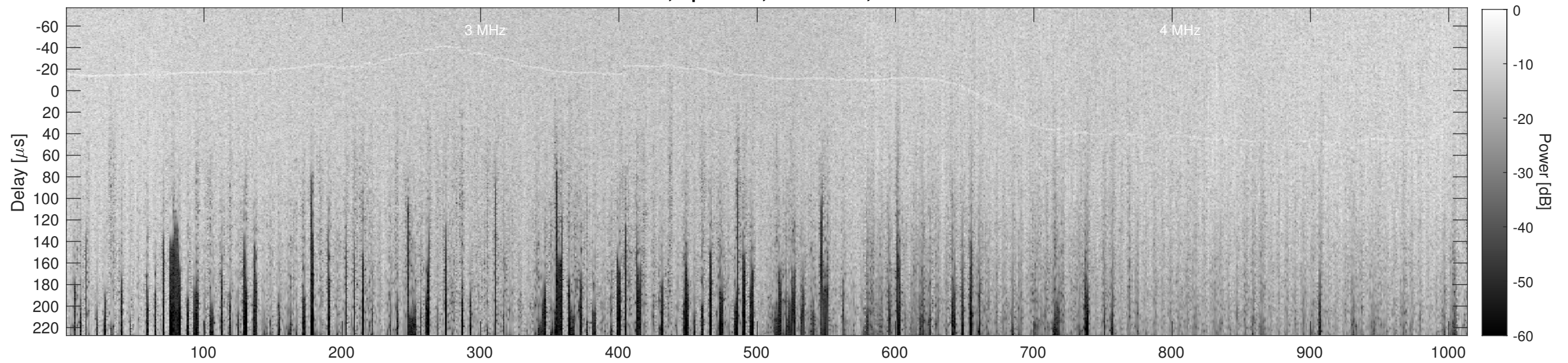
Orbit 10675, Cluttergram
