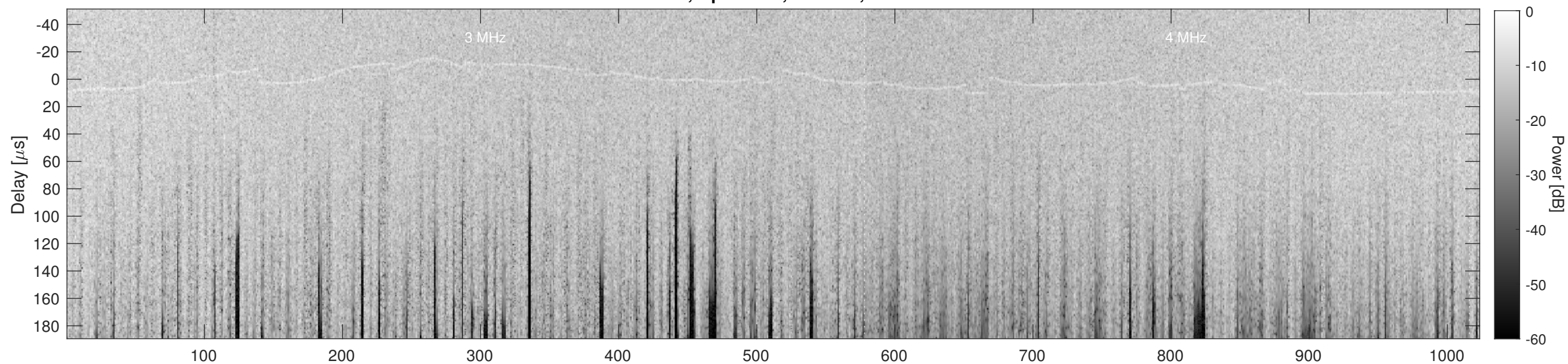
Orbit 10677, Cluttergram
