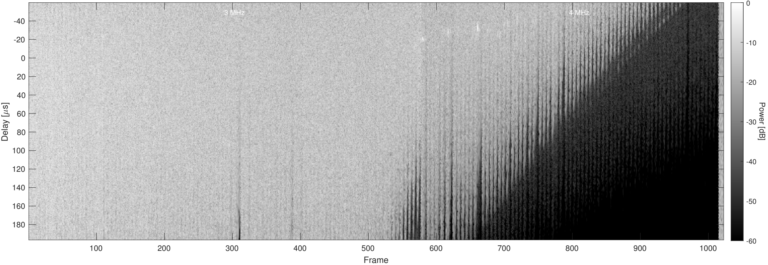
Orbit 10678, Chapman, No Window, Channel 2
