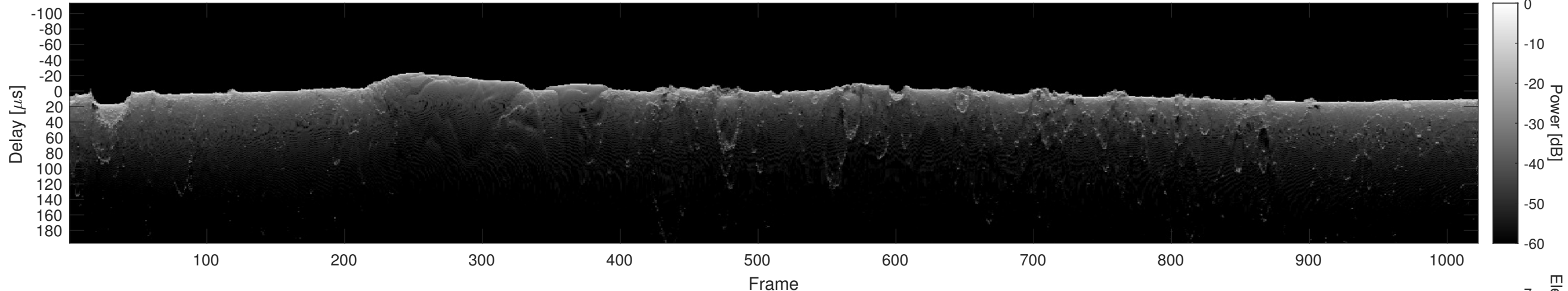
Orbit 10678, Cluttergram
