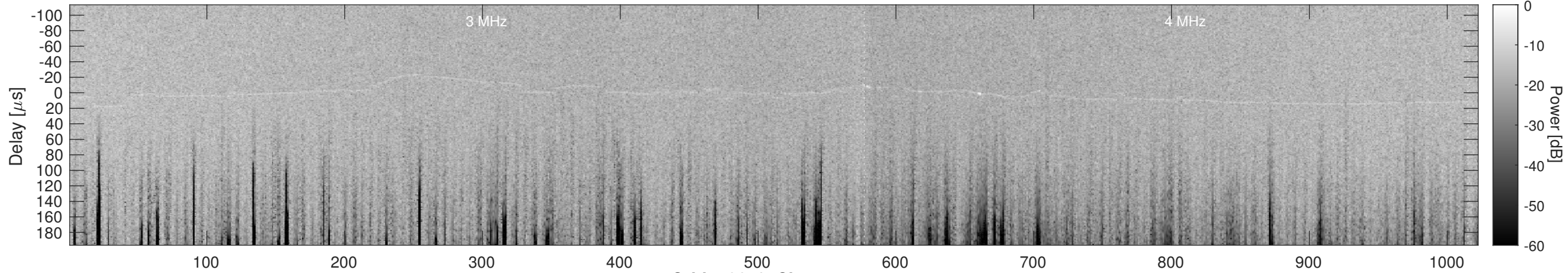
Orbit 10678, Cluttergram
