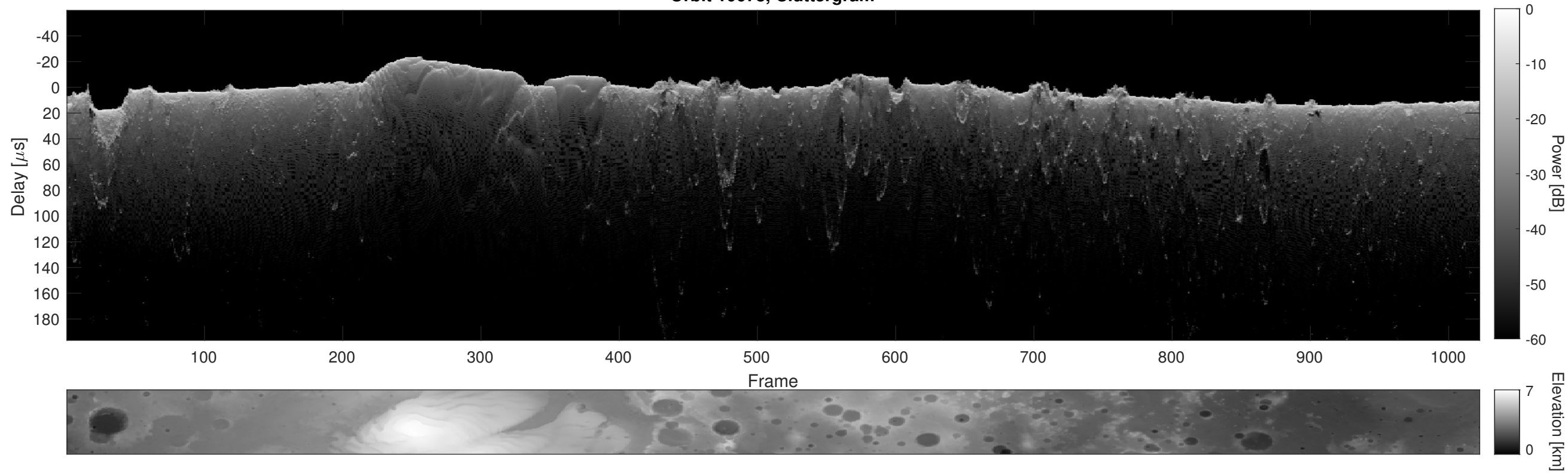
Orbit 10678, Cluttergram
