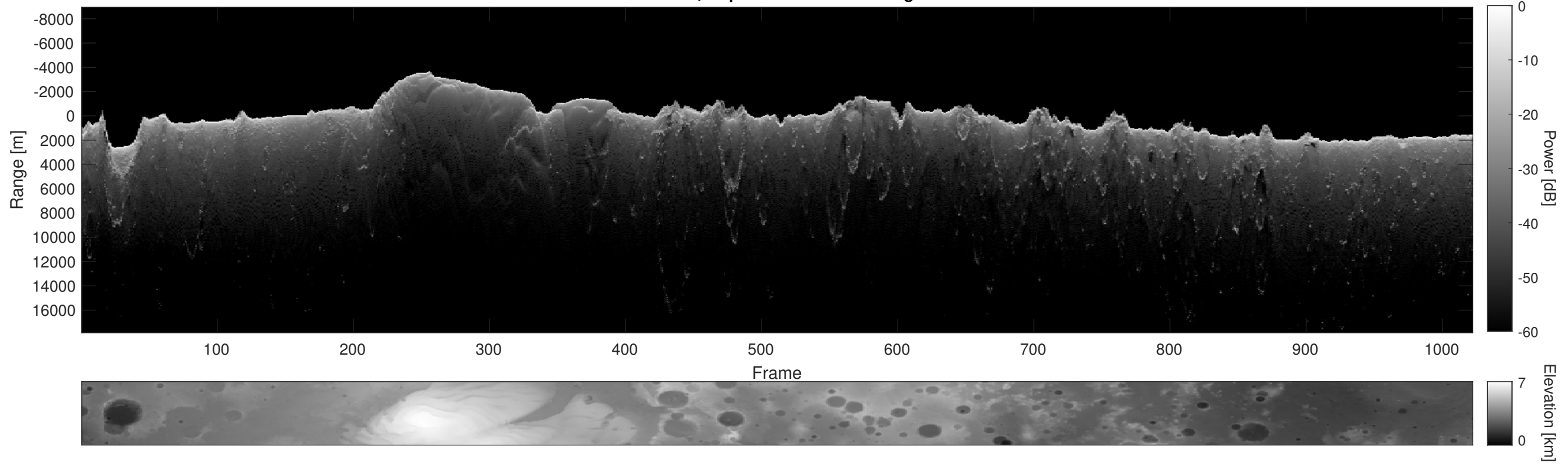
Orbit 10678, Depth-Corrected Cluttergram
