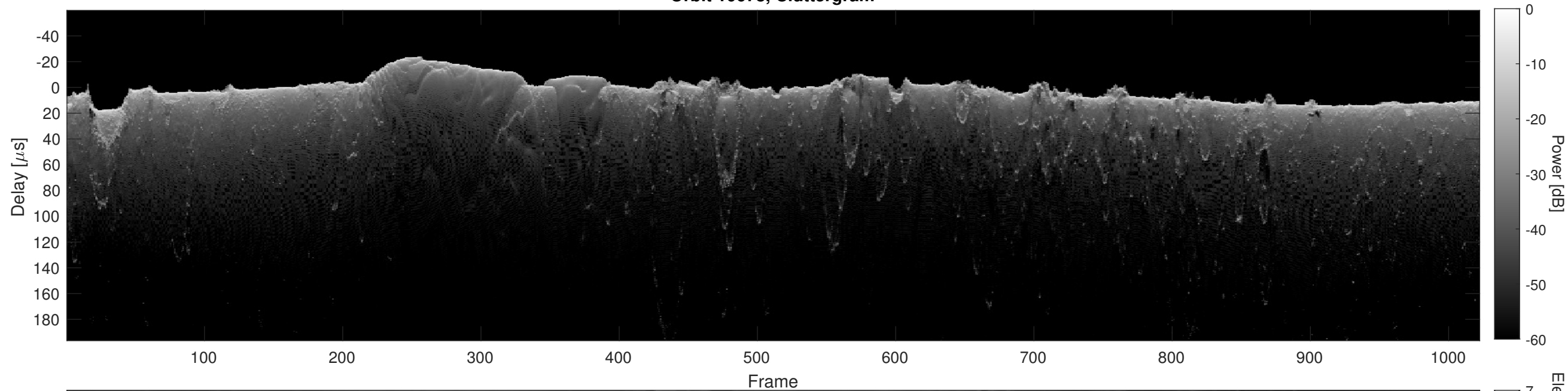
Orbit 10678, Cluttergram
