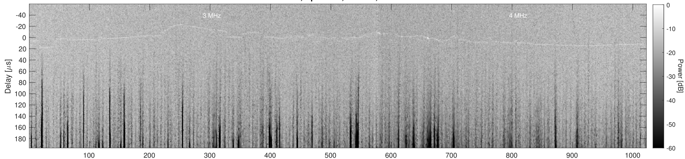
Orbit 10678, Cluttergram
