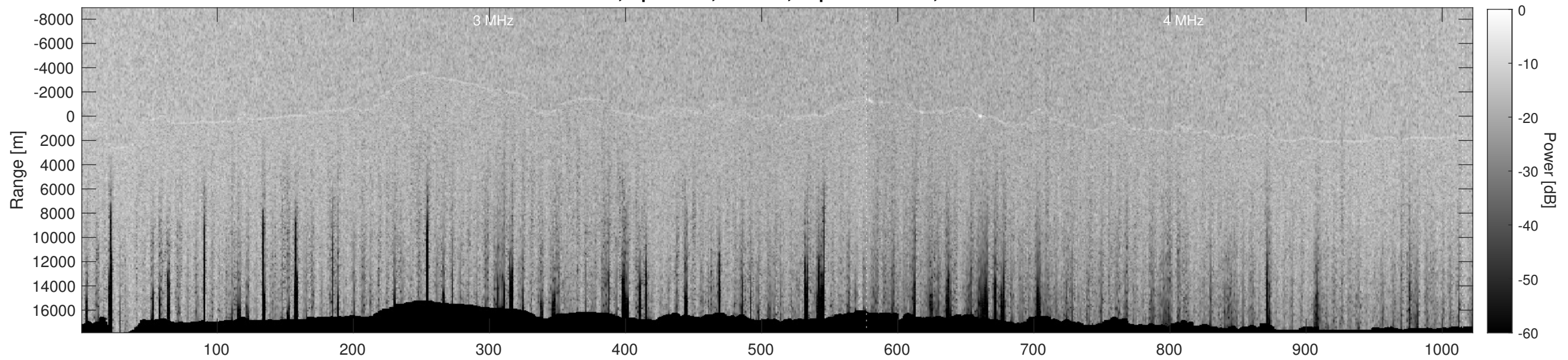
Orbit 10678, Depth-Corrected Cluttergram
