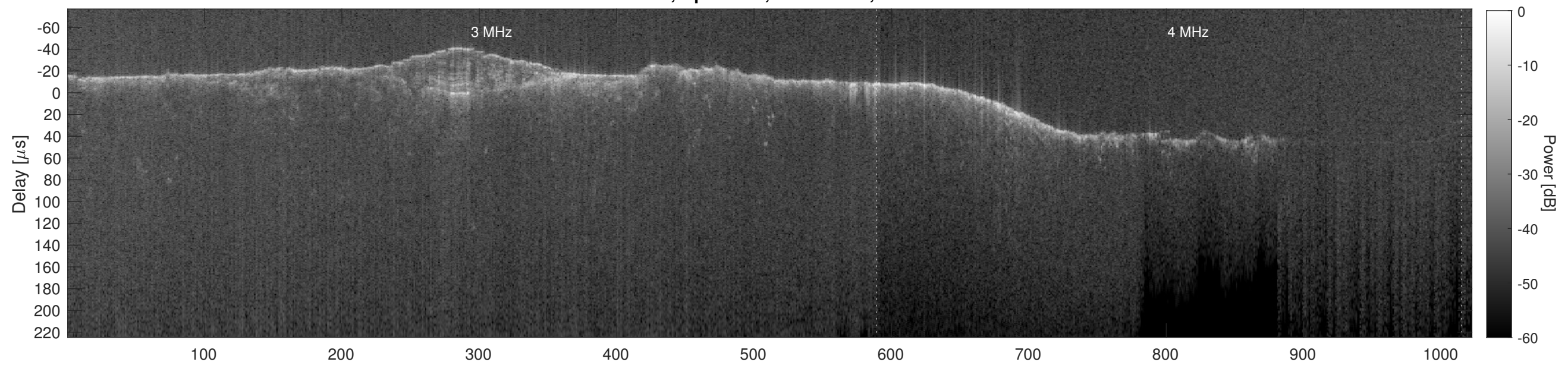
Orbit 10682, Cluttergram
