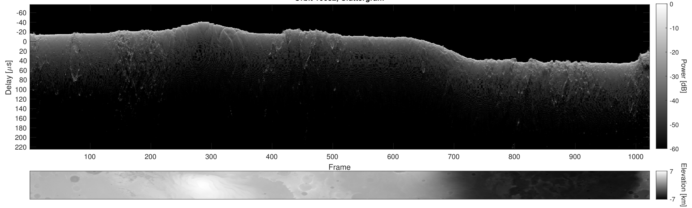
Orbit 10682, Cluttergram
