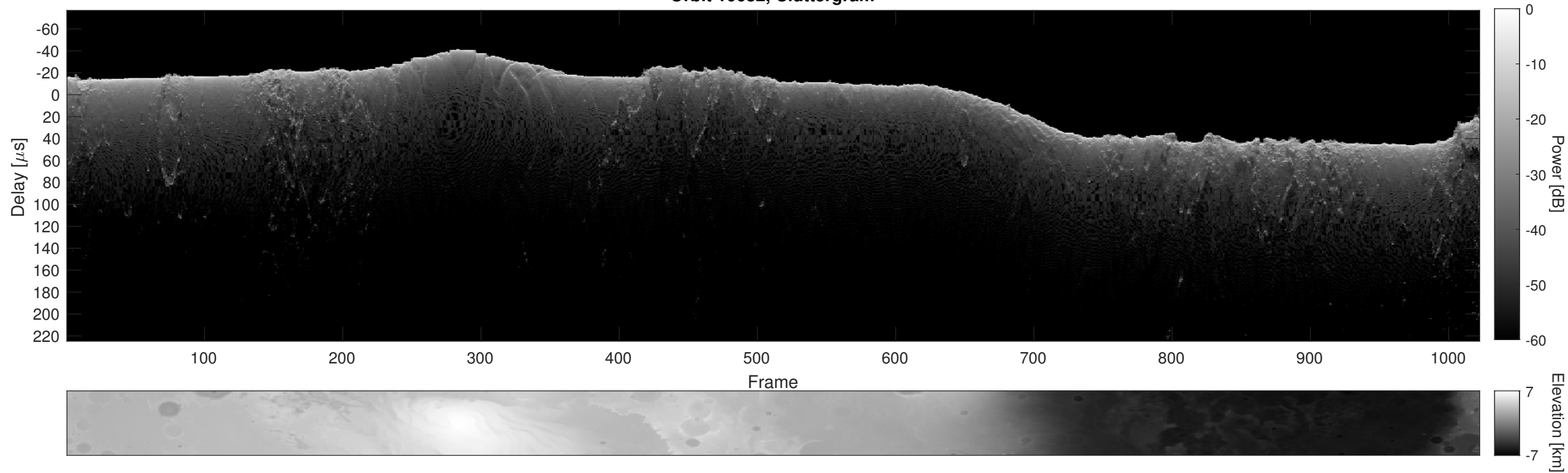
Orbit 10682, Cluttergram
