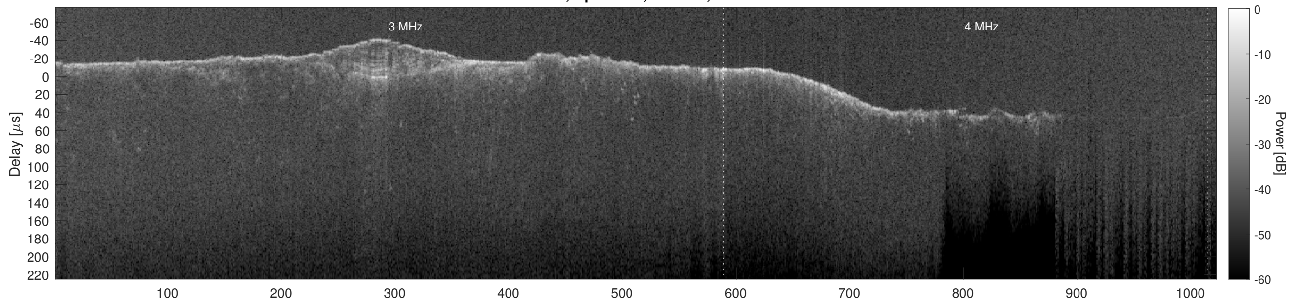
Orbit 10682, Cluttergram
